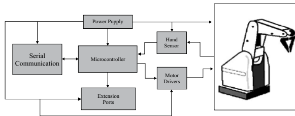
Figure 2 Block diagram of the electronic circuit of the robot
