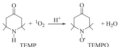
Figure 5 Oxidation of TEMP by singlet oxygen.
