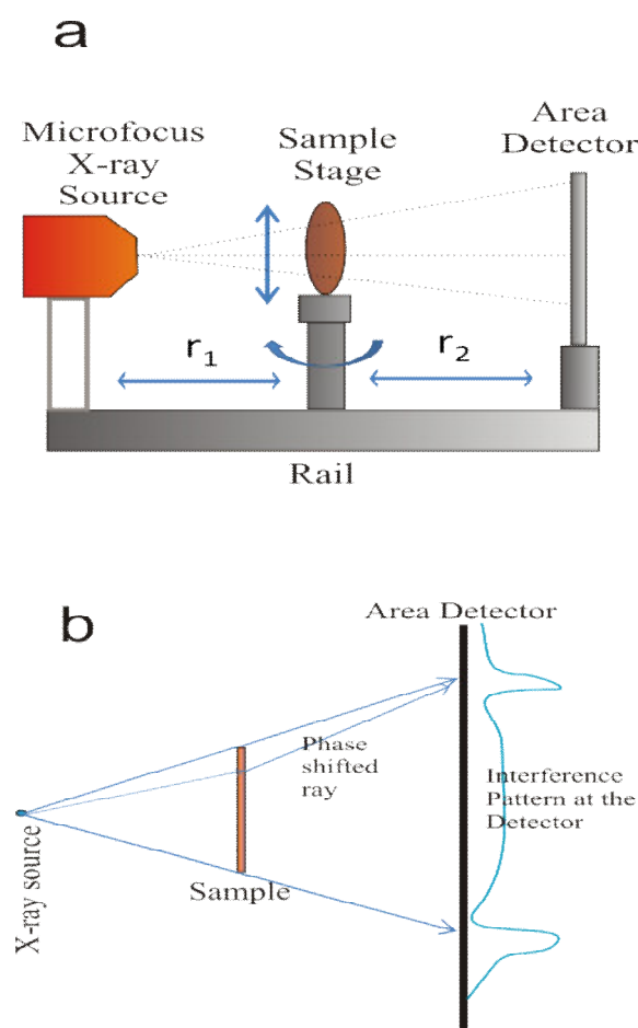
Figure 1. a) Experimental setup for microfocus X-ray imaging. b) Different regimes of imaging using phase contrast enhancement by a quasi-punctual X-ray source.
