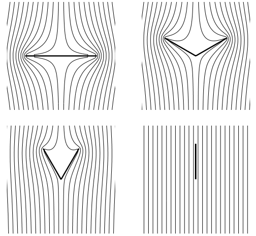
Figure 2. Magnetic field lines for bent thin strips in an external field B_a \parallel \hat{y} . Four bend angles are shown: \alpha = 0^\circ , corresponding to a flat strip, (top left); \alpha = 30^\circ (top right); \alpha = 60^\circ (bottom left) and \alpha = 90^\circ (bottom right).
