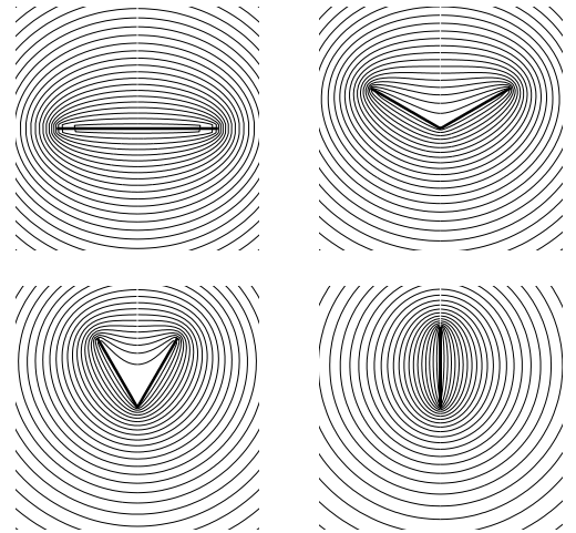
Figure 3. The same as Fig. 2, but for a transport current flowing along \hat{z} .
