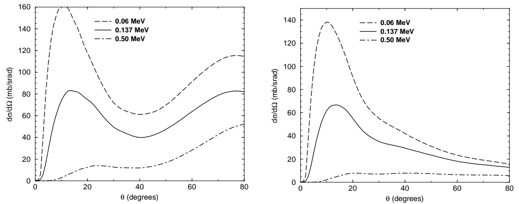
Figure 10. Dependence on the binding energy of the angular distribution for the breakup of {}^8\text{B} on {}^{58}\text{Ni} ( E_{lab} = 30 MeV): 1-step calculations on the lefthand side and full CDCC calculation on the righthand side. Dashed, solid and dot-dashed correspond to S_p = 0.06 MeV, S_p = 0.137 MeV and S_p = 0.50 MeV, respectively.
