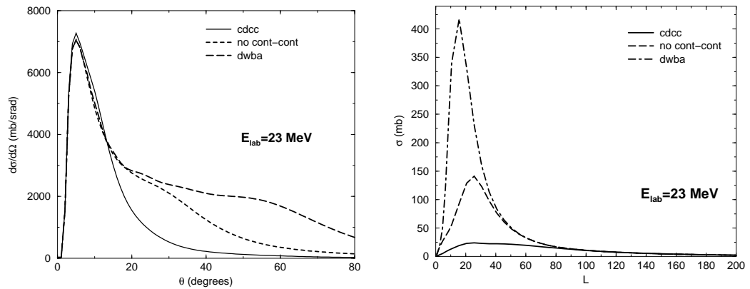
Figure 8. Same as before with E_{\text{lab}} = 23 \text{ MeV} .
