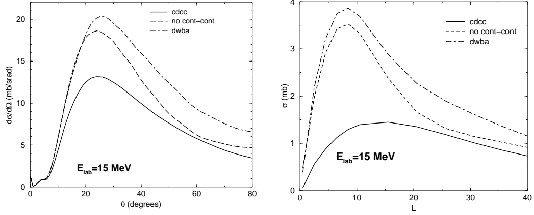
Figure 1. Angular distribution and L-distributions for the breakup of {}^8\text{B} on {}^{58}\text{Ni} , well below the barrier ( E_{\text{lab}} = 15 MeV): full CDCC calculations (solid line), truncated CDCC calculation where no continuum-continuum couplings are included (dashed line) and a 1-step calculation (dot-dashed line).
