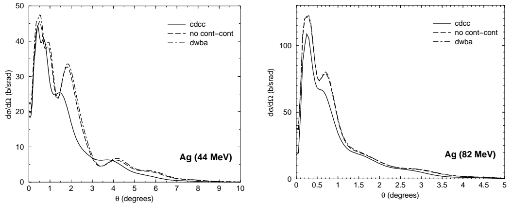
Figure 5. Angular distribution for the breakup of ^8\text{B} on ^{108}\text{Ag} , at both E_{\text{lab}} = 44, 82 MeV per nucleon: full CDCC calculations (solid line), truncated CDCC calculation where no continuum-continuum couplings are included (dashed line) and a 1-step calculation (dot-dashed line).
