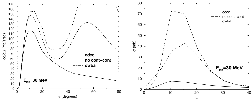
Figure 3. Same as before with E_{\text{lab}} = 30 MeV (on barrier).
