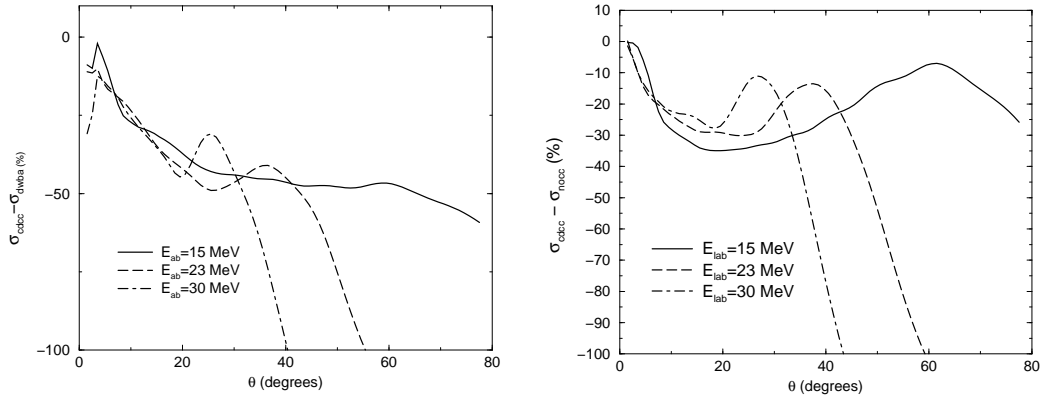
Figure 4. Relative importance of the continuum coupling for the breakup of ^8\text{B} on ^{58}\text{Ni} : the percentage difference between the full CDCC calculation and the 1-step results (left) and the percentage difference between the full CDCC calculations and the truncated CDCC calculation where no continuum-continuum couplings are included. The solid, dashed and dot-dashed lines correspond to the three energies E_{\text{lab}} = 15, 23, 30 MeV, respectively.
