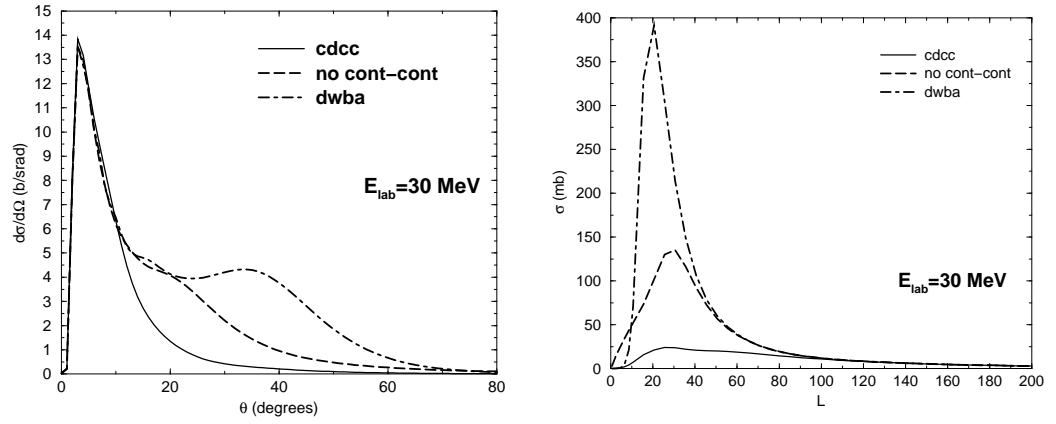
Figure 9. Same as before with E_{lab} = 30 MeV.
