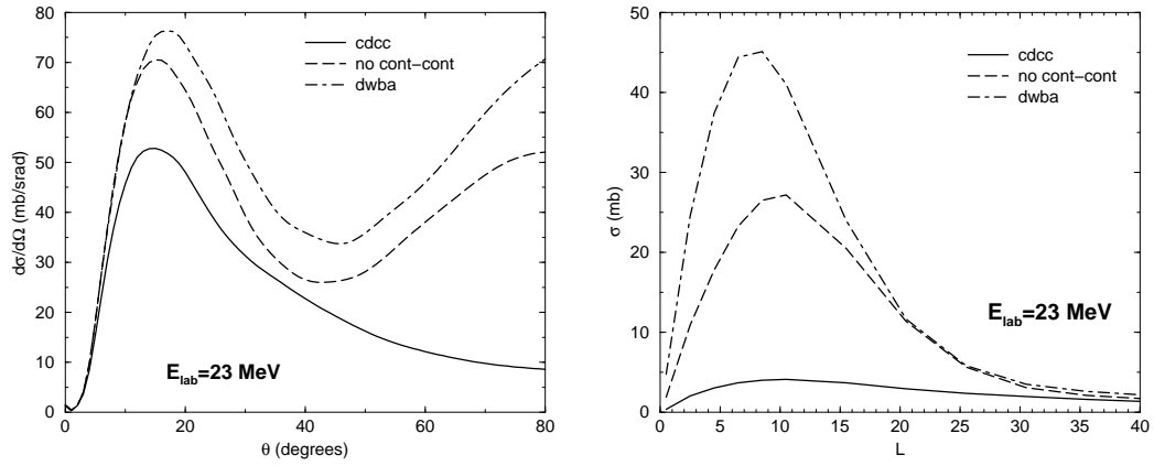
Figure 2. Same as before with E_{\text{lab}} = 23 MeV (on barrier).
