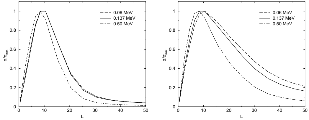
Figure 11. Dependence on the binding energy of the L-distribution for the breakup of {}^8\text{B} on {}^{58}\text{Ni} ( E_{\text{lab}} = 30 MeV): 1-step calculations on the lefthand side and full CDCC calculation on the righthand side. Dashed, solid and dot-dashed correspond to S_p = 0.06 MeV, S_p = 0.137 MeV and S_p = 0.5 MeV, respectively.
