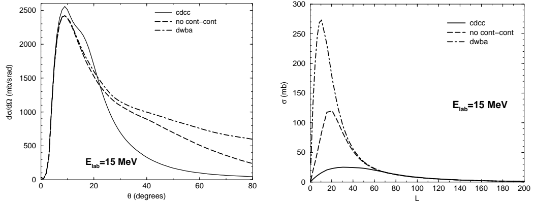
Figure 7. Angular distribution and L-distributions for the breakup of neutron ^8\text{B} on ^{58}\text{Ni} , well below the barrier ( E_{\text{lab}} = 15 \text{ MeV} ): full CDCC calculations (solid line), truncated CDCC calculation where no continuum-continuum couplings are included (dashed line) and a 1-step calculation (dot-dashed line).
