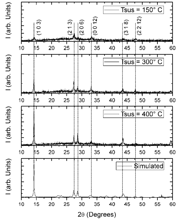
FIG. 5: Comparison of XRD pattern of In_2S_3 thin films deposited by co-evaporation on soda lime glass substrate varying the substrate temperature, with one XRD pattern simulated theoretically assuming that sample grown in the tetragonal \beta-In_2S_3 phase.
