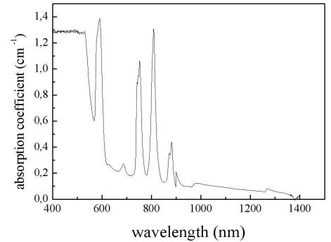
FIG. 2: Absorption spectrum of the \text{PbO-Bi}_2\text{O}_3\text{-Ga}_2\text{O}_3 glass doped with \text{Nd}_2\text{O}_3 (2 mm thickness).
