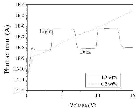
FIG. 6: Light and dark photocurrent of the \text{PbO-Bi}_2\text{O}_3\text{-Ga}_2\text{O}_3 with 0.2 and 1.0 wt% of \text{Nd}_2\text{O}_3 under illumination.
