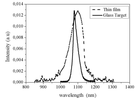
FIG. 5: Emission in the infrared region for the thin film and glass target of \text{PbO-Bi}_2\text{O}_3\text{-Ga}_2\text{O}_3 with 1.0 wt% of \text{Nd}_2\text{O}_3 .
