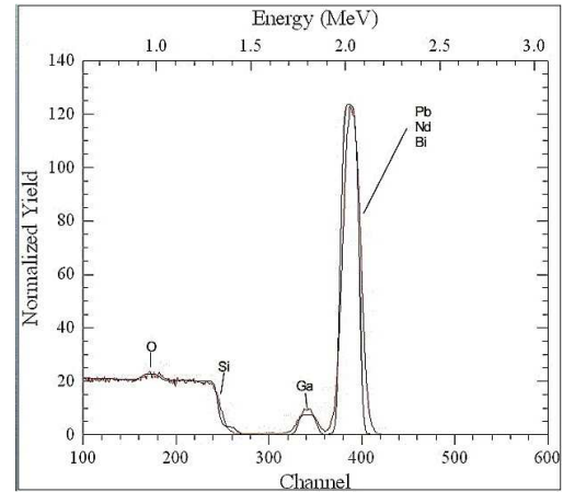
FIG. 1: RBS spectrum of the samples deposited during 2 hours.
