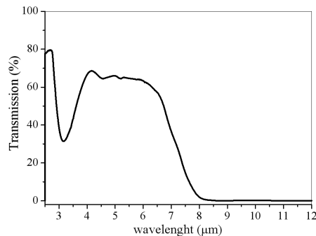
FIG. 3: Infrared transmission spectrum of the \text{Nd}_2\text{O}_3 doped \text{PbO-Bi}_2\text{O}_3\text{-Ga}_2\text{O}_3 glass target (1.0 wt% of \text{Nd}_2\text{O}_3 ).
