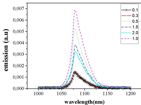
FIG. 4: Emission spectra of \text{PbO-Bi}_2\text{O}_3\text{-Ga}_2\text{O}_3 glasses doped with different concentrations of \text{Nd}_2\text{O}_3 (wt %).
