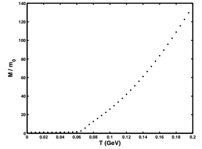
FIG. 5: The mass of the q -deformed quark fields, in units of the current quark mass m_0 = 5 \text{ MeV} , as a function of T for both q > 1 and q < 1 regimes. For small temperatures, M = m_0 .
