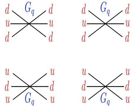
FIG. 1: Contact interactions generated by the mass term for the q -deformed fermion fields.
