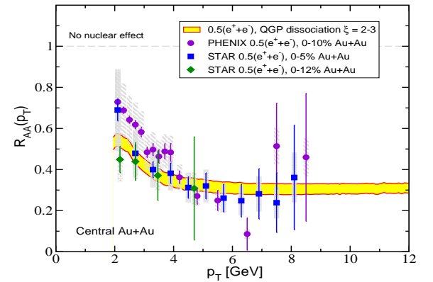
FIG. 3: Suppression of inclusive non-photonic electrons from D - and B -meson spectra softened by collisional dissociation in central Au+Au collisions. Data on non-photonic electron quenching from PHENIX [10, 16] and STAR [11, 14, 15] is also shown.
