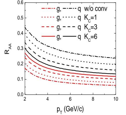
FIG. 3: (Color online) Nuclear modification factors for quark (upper lines) and gluon (lower lines) jets in central Au+Au collisions at \sqrt{s_{NN}} = 200 GeV as functions of transverse momentum without (dash-dotted lines) and with different enhancement factors K_C = 1 (dotted lines), K_C = 3 (dashed lines), and K_C = 6 (solid lines) for conversion scattering.
