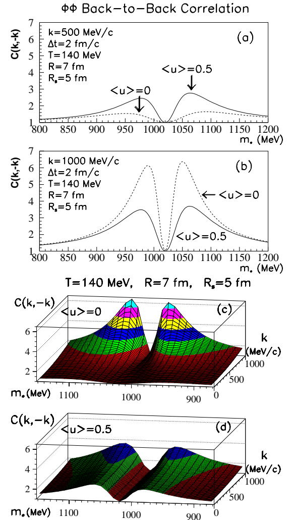
FIG. 3: (Color online) The plots in this panel are similar to the ones in Fig. 2. The main difference is that here we assumed that the mass-shift occurred only in a smaller part of the system volume. The back-to-back correlation is shown as a function of the shifted mass m_* on top, and as function of both m_* and the momentum of each particle ( \mathbf{k}_1 = -\mathbf{k}_2 = \mathbf{k} ), on bottom. The plots in parts (a) and (b) illustrate better the behavior of the BBC signal seen in parts (c) and (d), for |\mathbf{k}| = 500 MeV/c and for |\mathbf{k}| = 1000 MeV/c, respectively. In both cases, the dashed curve corresponds to \langle u \rangle = 0 and the solid curve, to \langle u \rangle = 0.5 . In (c), the 3-D plot without flow ( \langle u \rangle = 0 ) was considered, whereas in (d) a radial flow with v = \langle u \rangle r/R = 0.5 was included. The plots were extracted from Ref.[41].
