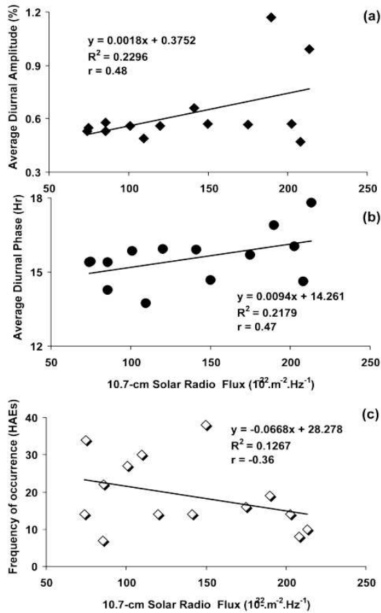
FIG. 3: The frequency of occurrence of days of high amplitude events for Deep River NM station along with annual average 10.7-cm solar radio flux for each year, during the period 1981-1994.
