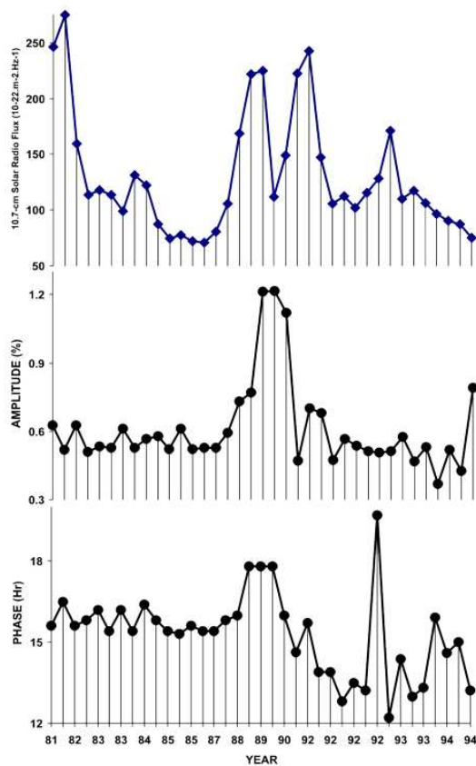
FIG. 1: The long-term variation of observed cosmic-ray diurnal amplitude (%) and the time of maximum (Hr) for each HAE event for Deep River NM station is shown as a function of solar cycle represented by 10.7-cm solar radio flux for the period 1981-1994.
