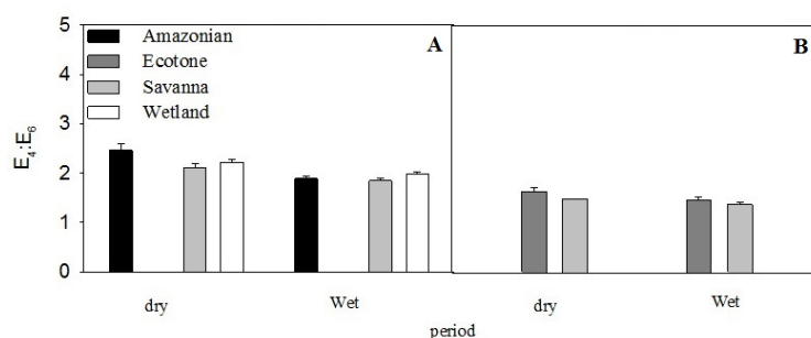
Figure 6: Mean ( \pm standard error) of E_4:E_6 in the different Biomes / Ecosystems. (A) Pasture (B) Soybean
