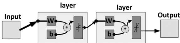
Figure 4. Schematic of neural network.
