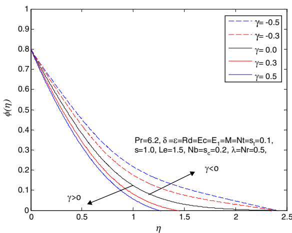
Fig. 19. Influence of \gamma on the concentration profile \phi(\eta) .
