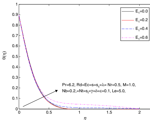
Fig. 13. Influence of E_i on the temperature profile \theta(\eta) .
