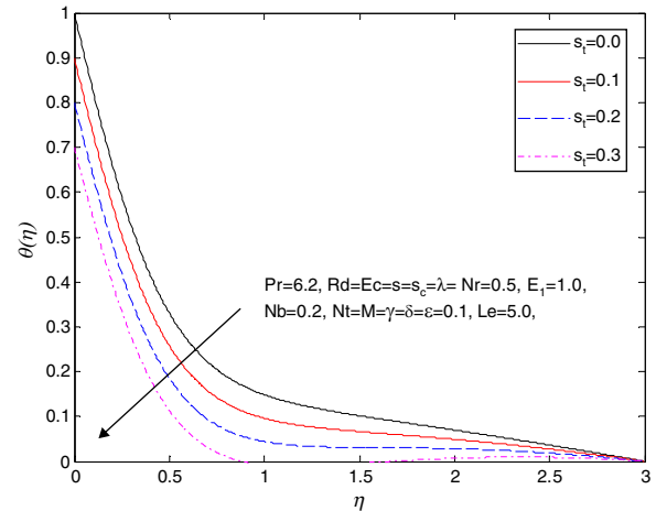
Fig. 14. Influence of s_i on the temperature profile \theta(\eta) .
