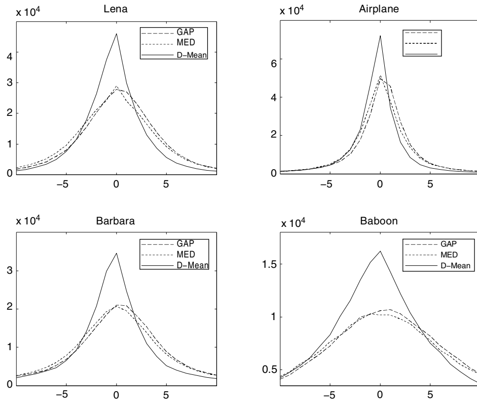
Fig. 2. Prediction-error histograms on standard images. X-axis and y-axis represent PE and its occurrence respectively.
