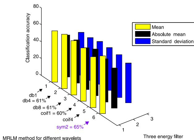
Fig. 16. MRLM (25 masks, L=3 ) for VisTex dataset.
