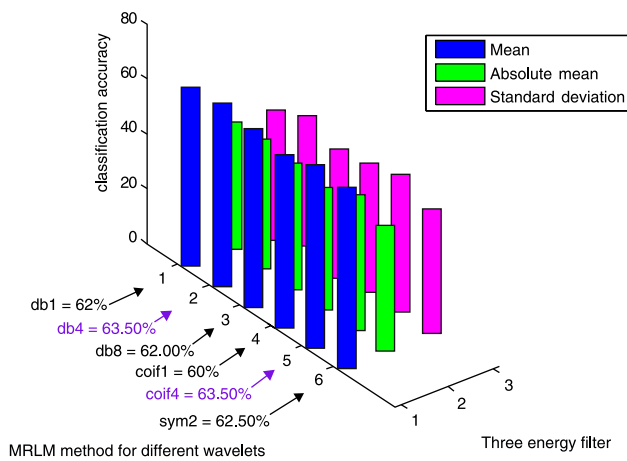
Fig. 14. MRLM (25 masks, L=1 ) for VisTex dataset.
