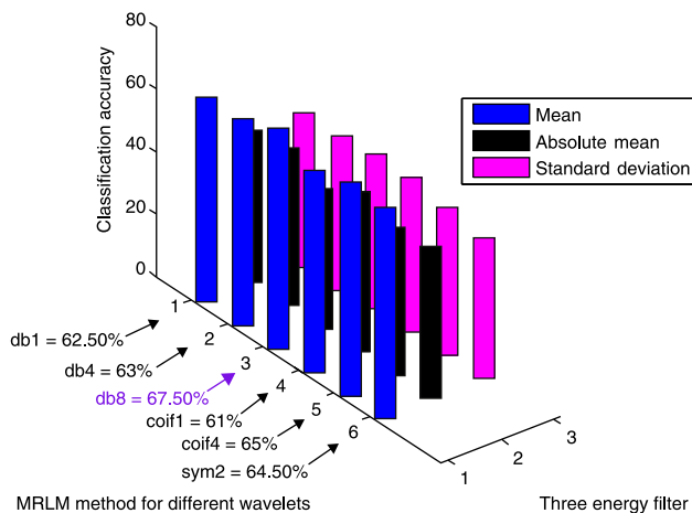
Fig. 15. MRLM (25 masks, L=2 ) for VisTex dataset.
