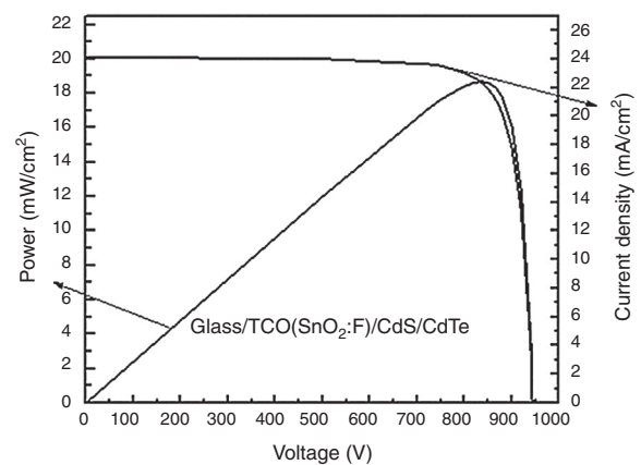
Fig. 15. Current density and power as functions of voltage for the 1 \mu\text{m} thick CdTe solar cell with S_n = 10^2 \text{ cm/s} .
