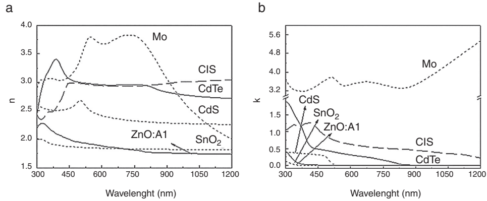
Fig. 2. (a) The refractive index and (b) the extinction coefficient for ZnO:Al, Mo, CIS, CdS, SnO 2 and CdTe films.
