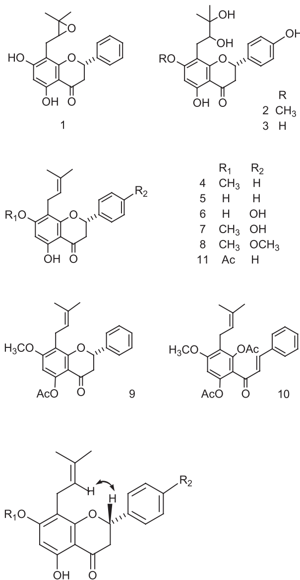
Fig. 1. H-2 / H-2'' NOESY correlation
