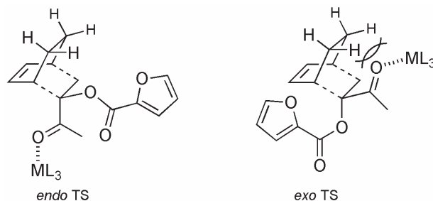
Fig. 10. Possible steric interactions at the endo and exo transition states (TS) in the Diels-Alder cycloadditions of olefin 3a and cyclohexadiene ( 12 ).
