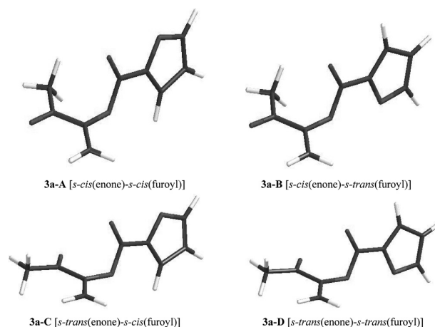
Fig. 3. Optimized geometries (HF/6-31G*) of olefin 3a for the non-planar conformations A-D.
