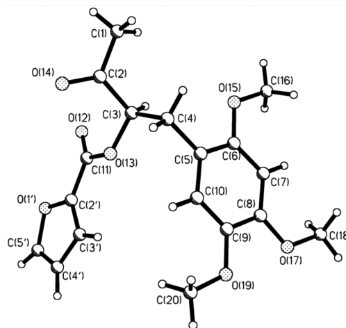
Fig. 6. X-ray structure of captodative olefin 8 (ellipsoids with 30% probability)
