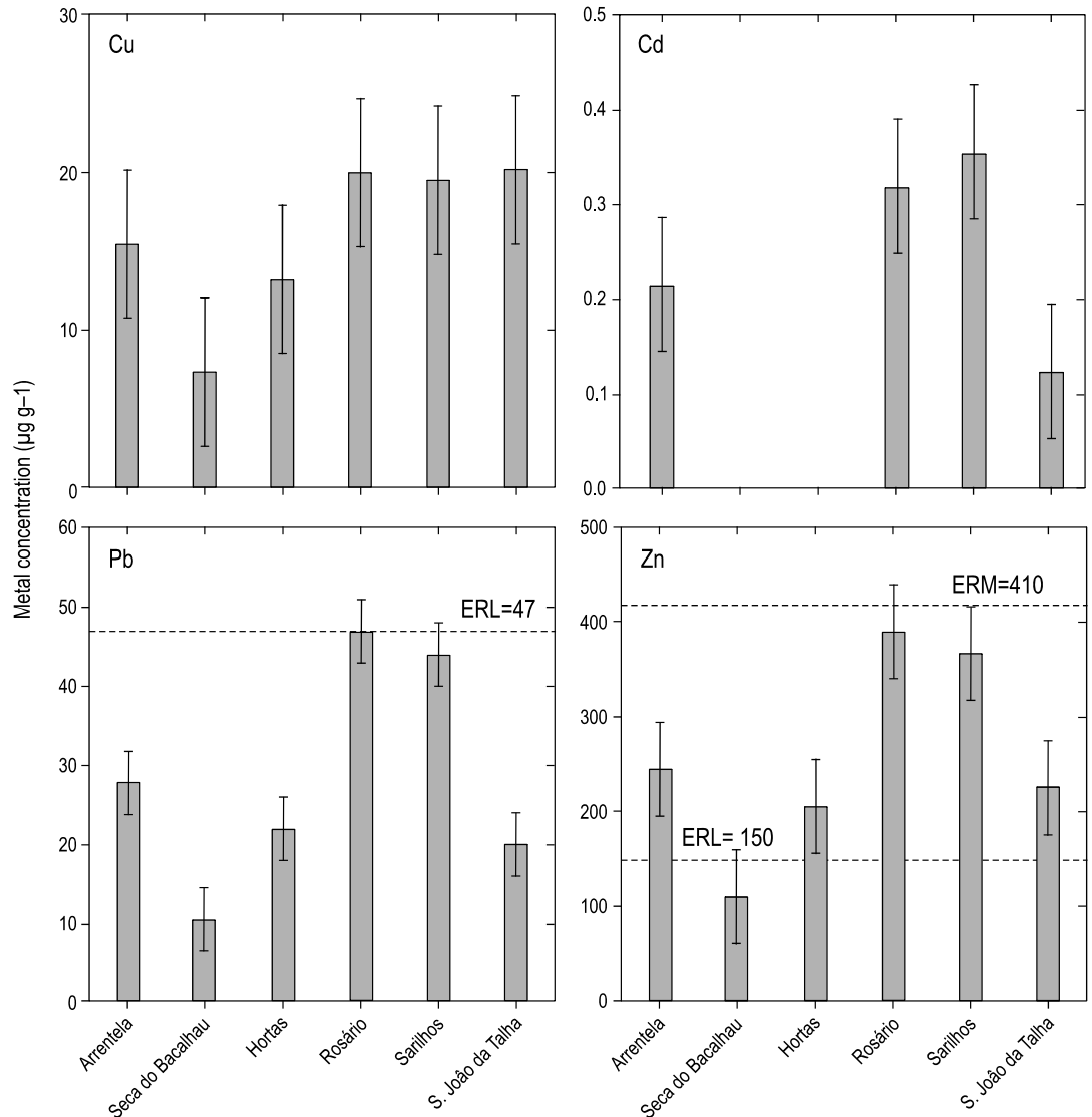
Figure 2. Heavy metal (Cu, Cd, Pb, and Zn) contents in sediment samples from the six mudflats sampled (standard deviation above bars). Dashed lines represent the effect range low (ERL) and the effect range median (ERM) for each metal.
