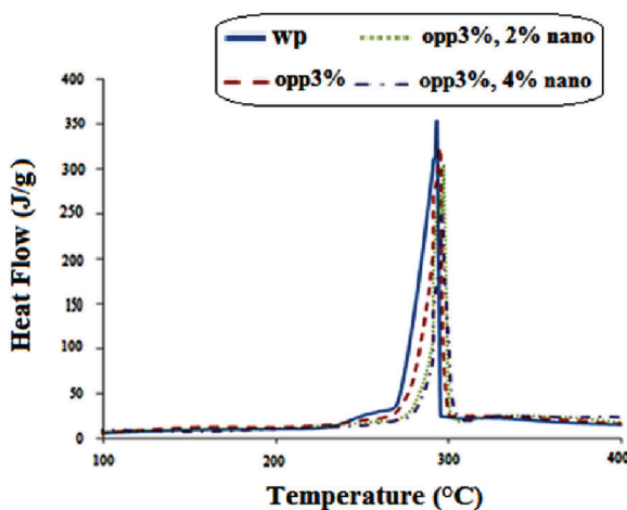
Figure 5. DTA curves of the samples.
