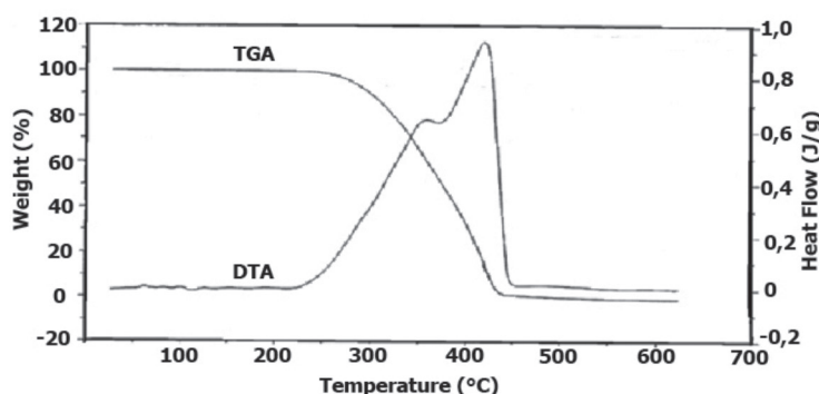
Figure 2. TGA and DTA curves of non-oxidized polypropylene.
