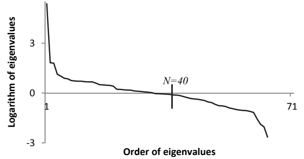
Figure 2. Optimum value of N . Beyond this value ( N=40 ), the logarithm of eigenvalues are negative.
