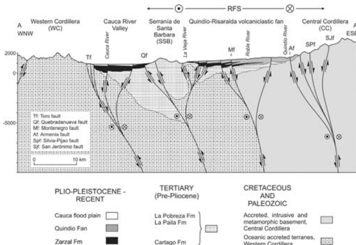
FIGURE 4 | Simplified geological cross-section from Western to Central Cordilleras (profile AA' in Figure 3A) after Alfonso et al. (1994), Guzmán et al. (1998), INGEOMINAS (1999), Paris et al. (2000), Taboada et al. (2000), Suter (2003), Gallego et al. (2005), USGS (2005). This interpretation allows for localized zones of subsidence (Cauca and Quindío-Risaralda Basins) within a regional, compressional tectonic regime.
