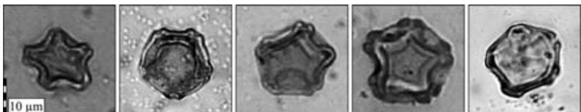
FIGURE 10 | Alnus pollen grains encountered in Zarzal Formation clays (see Figures 7, 8 and 9). The first record of this tree in Colombia dates back to less than 1 Ma ago (Hooghiemstra and Cleef, 1995).
