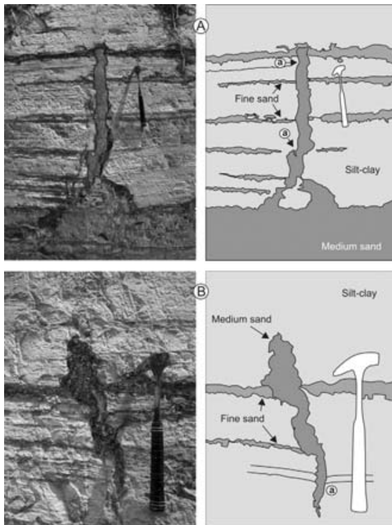
FIGURE 13 | Soft-sediment deformations in Zarzal Formation (modified after Neuwerth et al., 2006): A) rooted, vertical, medium-grained sand dyke intruding silty clays; this intrusion is partially controlled by fractures (a). B) disconnected, subvertical, medium-grained sand dyke showing downward bending of intruded, fine-grained sediments (a) in the lower part.
