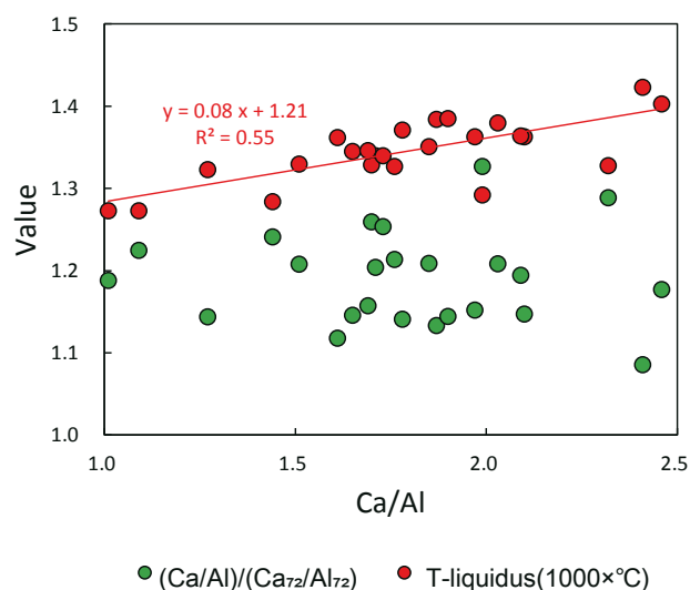
FIGURE 10. Variations of T-liquidus and (\text{Ca}/\text{Al})/(\text{Ca}_{72}/\text{Al}_{72}) with increasing Ca/Al. The red continuous line represents the calculated trend line of T-liquidus.
