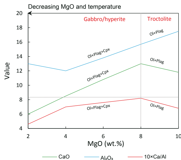
FIGURE 5. Liquid Lines of Descent (LLD) illustrated by \text{Al}_2\text{O}_3 , \text{CaO} and \text{Ca/Al} in anhydrous mid-ocean ridge basalt melts (after Niu, 2005; Niu and O'Hara, 2008). The gray vertical continuous line represents the critical point of gabbro/hyperite crystallization at \text{MgO} = 8\text{wt.}\% . The gray horizontal continuous line represents the maximum value of \text{Ca/Al} (<0.85) during fractional crystallization processes.
