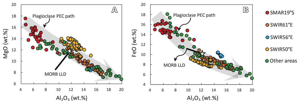
FIGURE 4. Plots of \text{Al}_2\text{O}_3 versus A) \text{MgO} and B) \text{FeO} in plagioclase-hosted MIs from SWIR (Font et al. , 2007) and SMAR19°S. The plagioclase PEC path (gray arrows), a hypothetical near-primary melt composition (white stars), and MORB Liquid Lines of Descent (LLD) (black solid lines) are shown for comparison (after Neave et al. , 2015).
