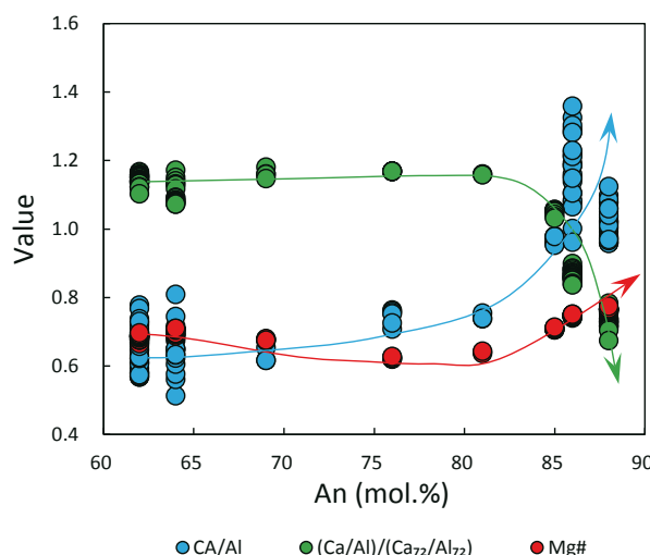
FIGURE 9. Variations of \text{Ca}/\text{Al} , (\text{Ca}/\text{Al})/(\text{Ca}_{72}/\text{Al}_{72}) and \text{Mg\#} with increasing An content in host plagioclases. Continuous curves represent the general variability trends.
