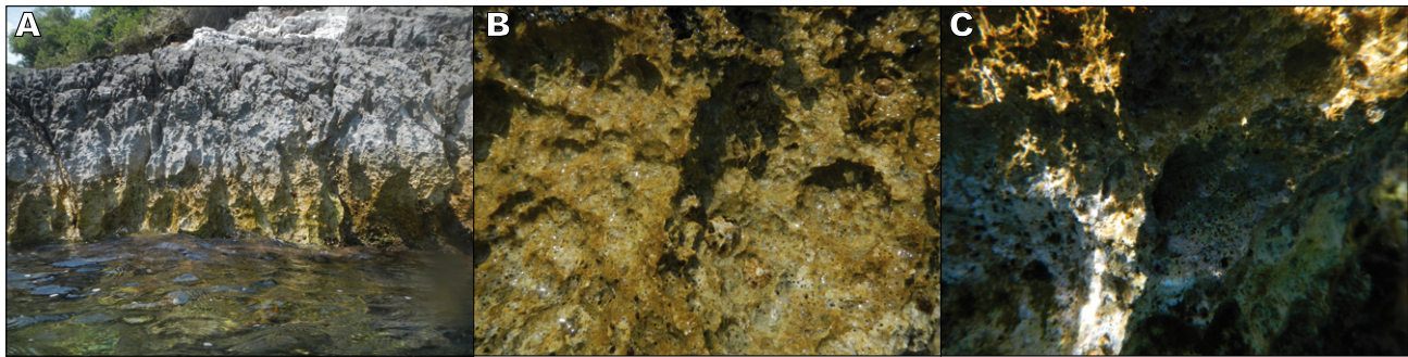
FIGURE 6. Overprinted bioerosion features – evidence of alternating subsidence and uplift events A) holes of subtidal boring bivalves overprinted by supratidal coastal karren; B) subtidal sea urchin boreholes emerged into the supratidal zone, overprinted by coastal karren; C) dark spot: subtidal sea urchin borehole as seen in the roof of uplifted marine notch. For more details see also Table 5.
