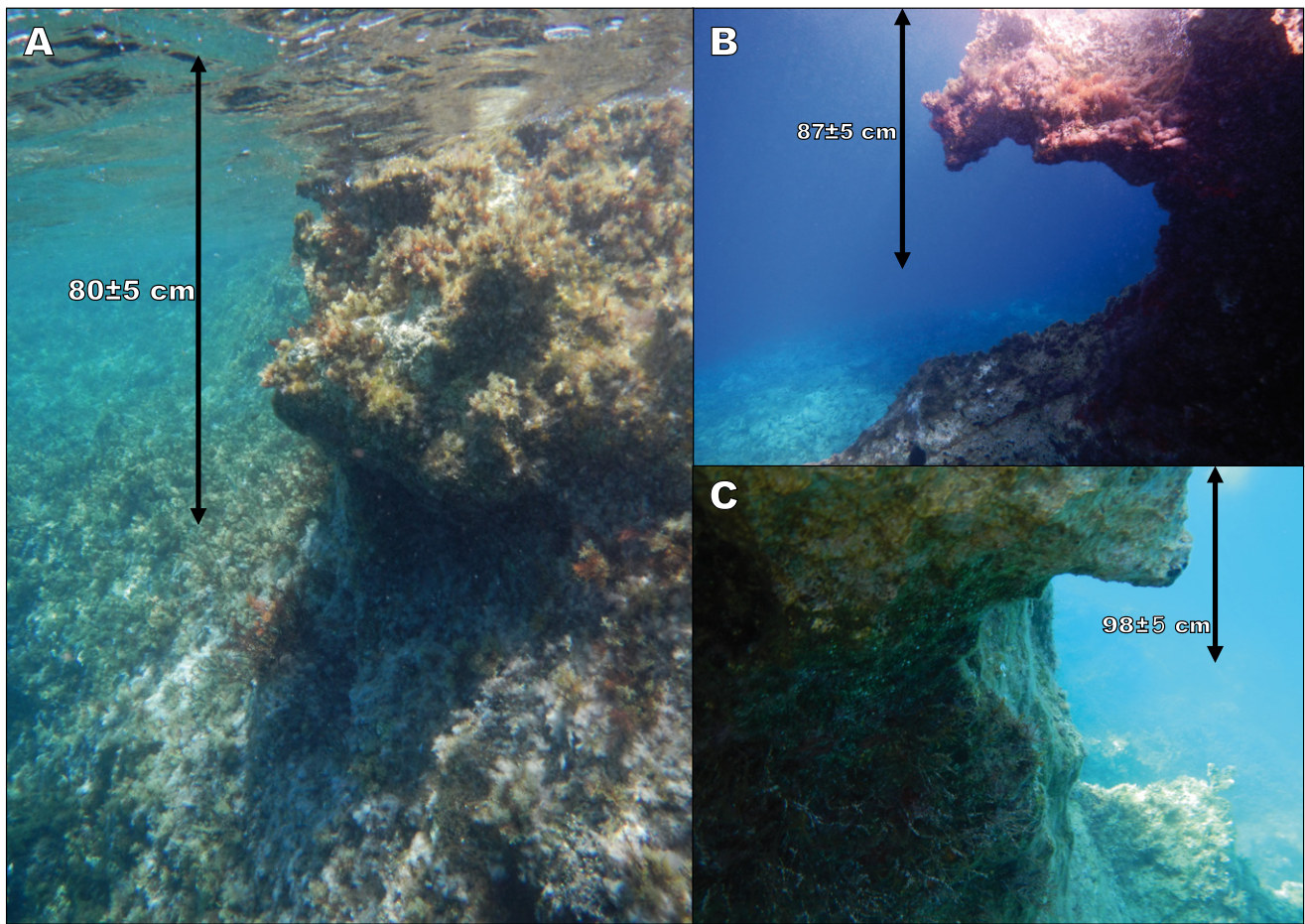
FIGURE 5. A) Submerged shoreline at about -80 \pm 5 cm at Fiscardo peninsula at site KE36.2. The upper part of the arrow starts from SL. B) Submerged shoreline at about -87 \pm 5 cm at Fiscardo peninsula at site KE42.2. A living sea urchin is hiding in its own hole just below the notch. C) Submerged shoreline at about -98 \pm 5 cm at Fiscardo peninsula at site KE41.2. The upper part of the arrow starts from SL.
