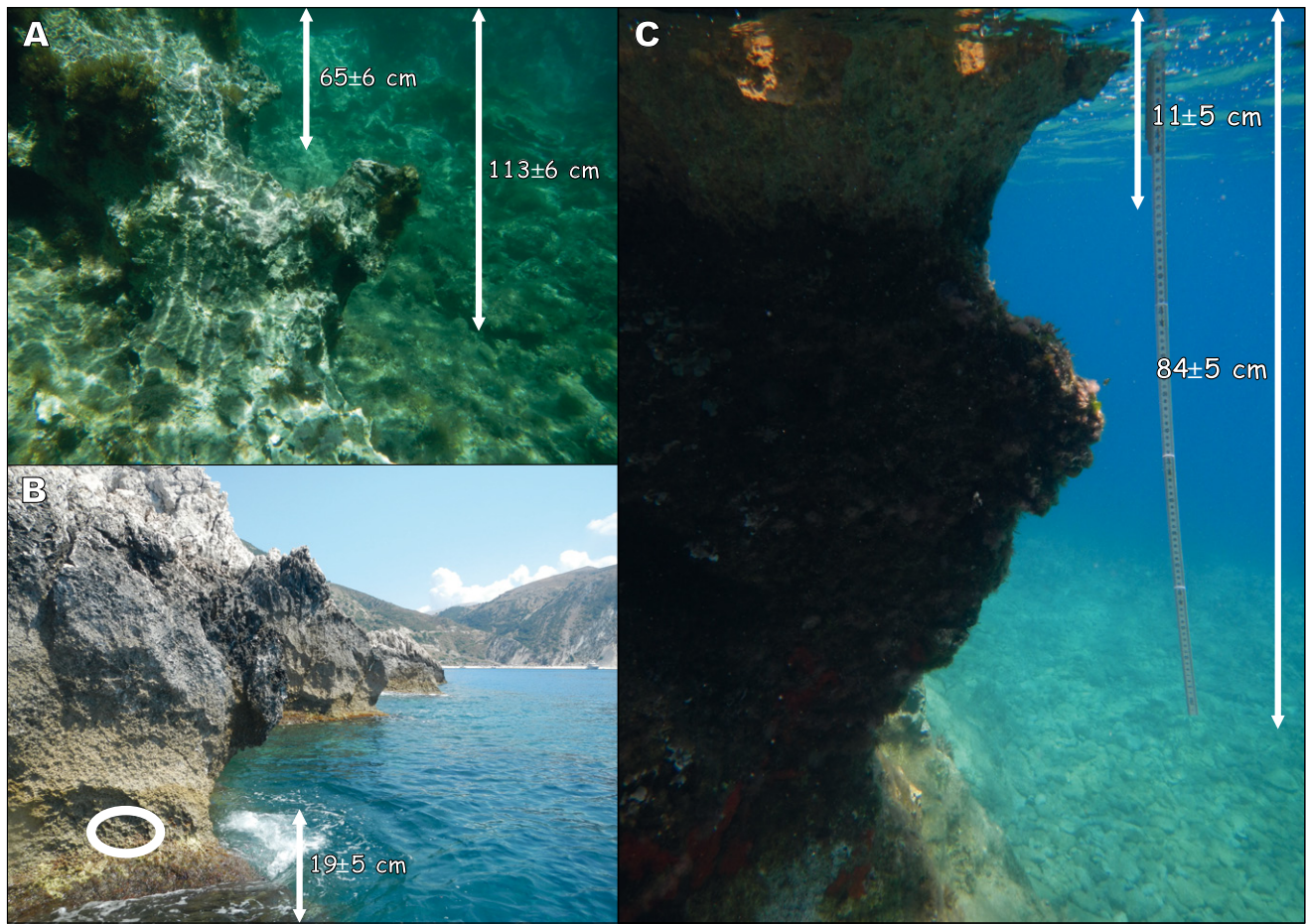
FIGURE 4. A) Shoreline E at Ithaca island at about -113\pm 6 cm located at site ITH11.2. Shoreline A is also visible above shoreline E at about -65\pm 6 cm. The upper part of the arrow starts from Sea Level (SL). B) Emerged shoreline at about +19\pm 5 cm located at site KE39.2. C) Submerged shoreline at about -11\pm 5 cm at Fiscardo peninsula at KE4.2, while below another shoreline at about -84\pm 5 is also visible (KE4.3). The upper part of the arrow starts from SL.
