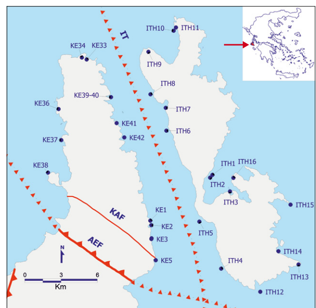
FIGURE 1. Surveyed area. Dots represent the sites discussed in the text and listed in Tables II and III. Site names are also shown in this map, while the measurements and characteristics of each of these are listed in Tables II and III. Different lines depicted in this map correspond to the main faults in the study area, based on Sorel (1976) and Stiros et al. (1994). Specifically, AEF is the Agia Ephemera Fault and its inferred extension offshore, a major active reverse fault, KAF is the Kalon Anticline Fault, satellite fault in the hanging wall of the main fault and IT is the Ionian Thrust.
