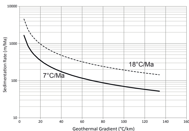
FIGURE 8. Modified Clayton's chart showing the equivalence in term of heating rate. The optimal geological condition for the biogenic gas generation and preservation in the geological system is comprised between both curves.
