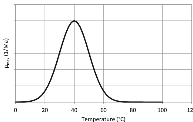
FIGURE 2. Example of temperature dependency for \mu_{\max} .
