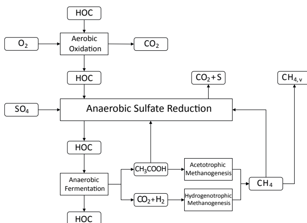
FIGURE 1. Reaction scheme used in the 1D microscopic model.
