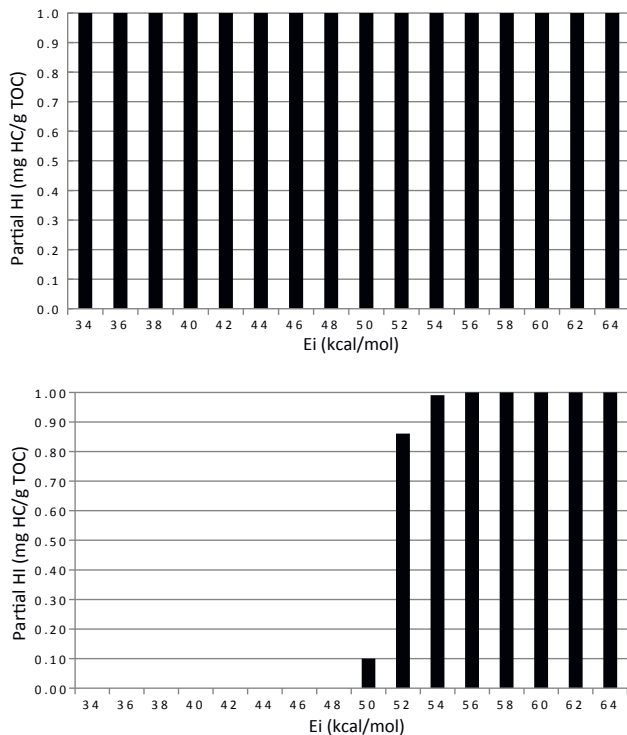
FIGURE 9. Artificial maturity experiment on a synthetic sample (A) with uniform distribution of partial potential and A = 3.1 \cdot 10^{15} \text{ s}^{-1} . At maturity equivalent to R_o = 0.6\% (B) all the partial potentials have been totally consumed for activation energy below 50 kcal/mol.
