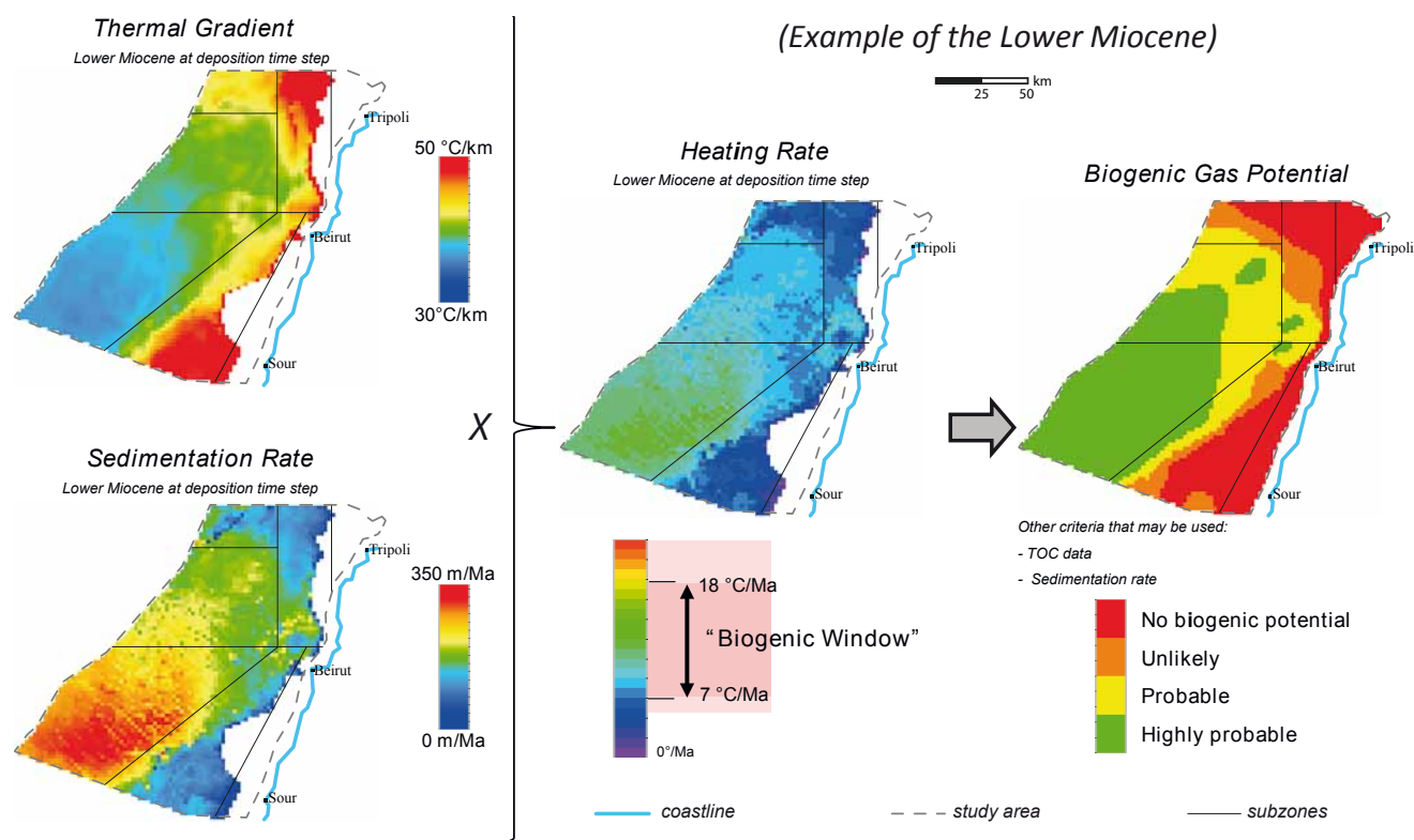
Figure 11. Illustration of the methodology that identify, for a given layer, the area that may produce microbial gas. The thermal gradient is calculated in the uppermost layer of the model, the average thermal gradient in the basin is much lower around 22°C/km.
