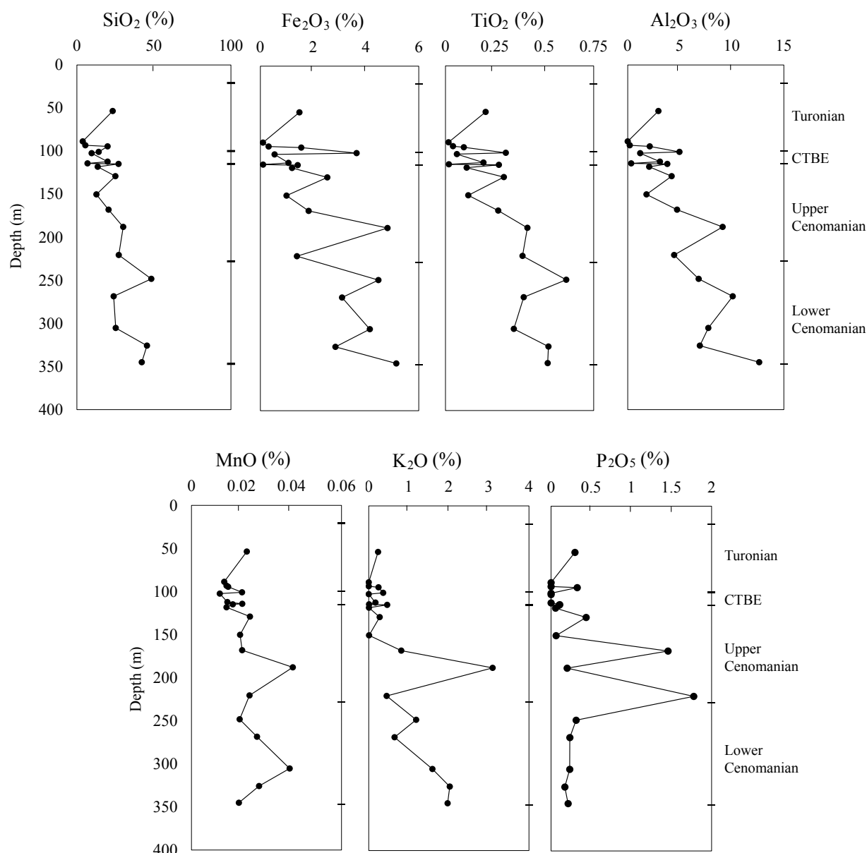
FIGURE 6. Elemental data versus depth shows increase in silicate and rutile forming elements with depth. It also shows a strong increase in P_2O_5 before the CTBE.
