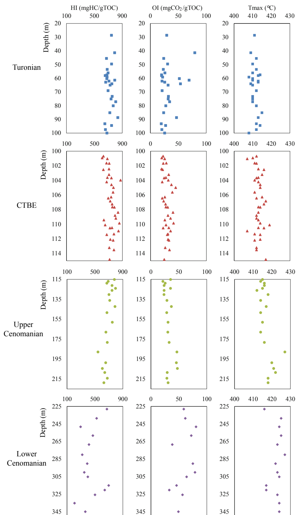
FIGURE 9. Rock Eval HI, OI and T_{max} versus depth plot. It shows the apparent difference between the Cenomanian to Turonian source rocks. On the basis of microscopic observations the T_{max} shift is interpreted to be caused by a change in the organic facies rather than thermal maturity.
