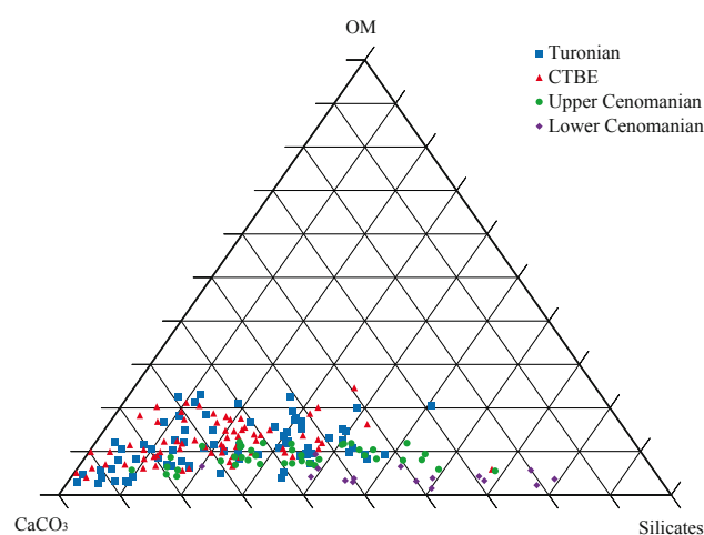
FIGURE 16. OM-CaCO 3 -Silicates ternary diagram (modified after Littke, 1993) showing that the best organic preservation is achieved at CaCO 3 concentration between 45 to 80%.
