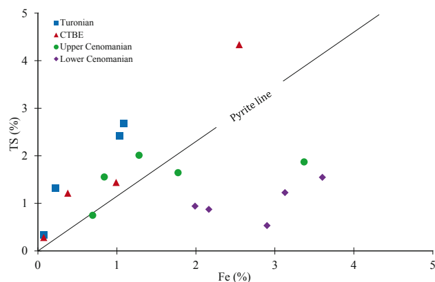
FIGURE 15. TS versus Fe shows that the majority of the samples from Cenomanian to Turonian are plotted above the Pyrite line indicating that the sulfur in these samples is present in other form than pyrite.
