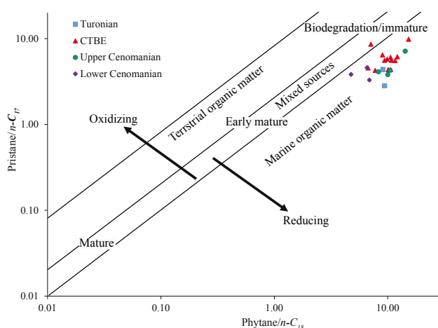
FIGURE 12. Pr/C 17 vs. Ph/C 18 diagram suggests marine and thermally immature organic matter for all sample. The classification method is from Shanmugam (1985).
