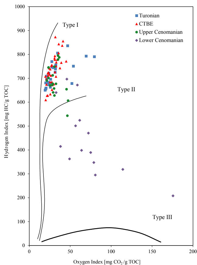
FIGURE 8. Pseudo van Krevelen diagram of bulk Rock Eval-6 samples of the various stratigraphic intervals.
