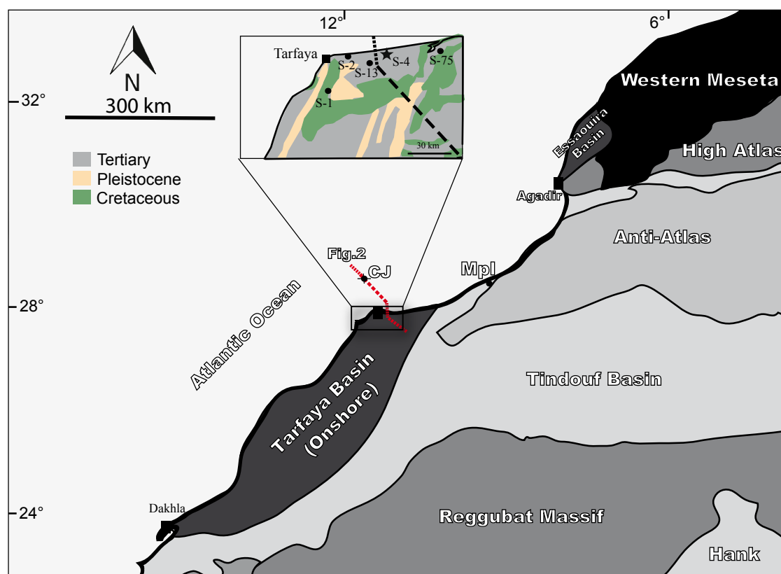
FIGURE 1. Overview map of the Tarfaya Basin showing the location of the studied well (S-4) and some of the previously studied wells (modified after Michard et al. , 2008). Surface geology in the small map modified after Saadi et al. (1985). CJ: Cap Juby well.
