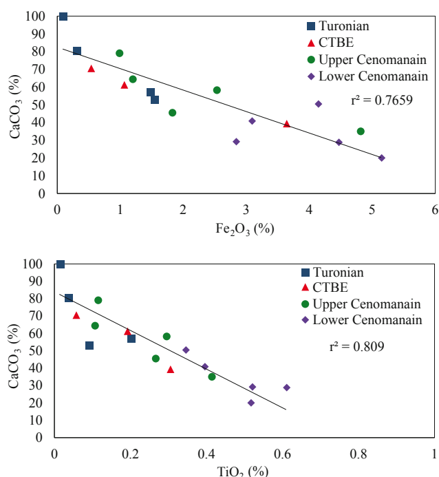
FIGURE 7. \text{CaCO}_3 versus \text{Fe}_2\text{O}_3 and \text{TiO}_2 Cross plots show inverse relationship in all studied intervals.
