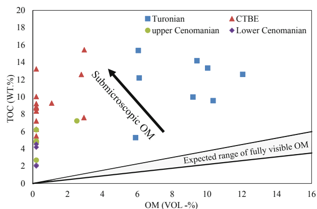
FIGURE 11. Organic matter volume vs. TOC weight percent. The samples that show very low visible organic matter were assigned as 0.2% for the sake of simplicity.
