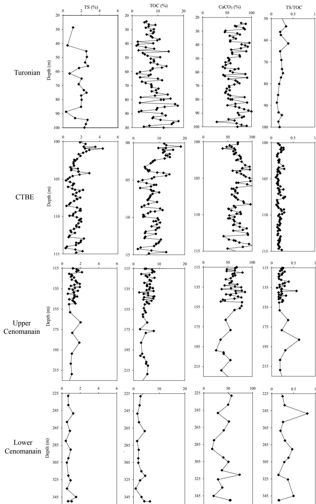
FIGURE 4. Depth plots TS, TOC, CaCO 3 and TS/TOC ratio of all stratigraphic units.
