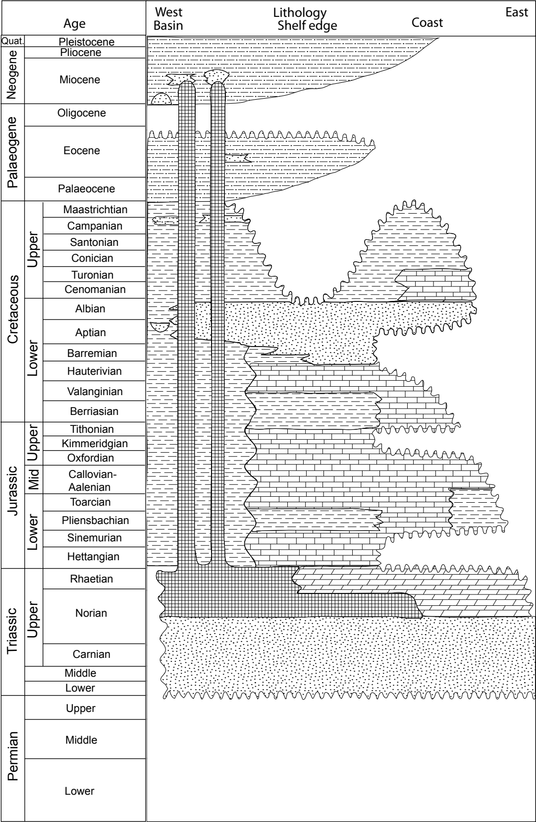
FIGURE 3. Stratigraphic column representing the common lithologies in the Tarfaya Basin from coastal to deep marine areas (modified after Davison, 2005; Sehr, 2014).
