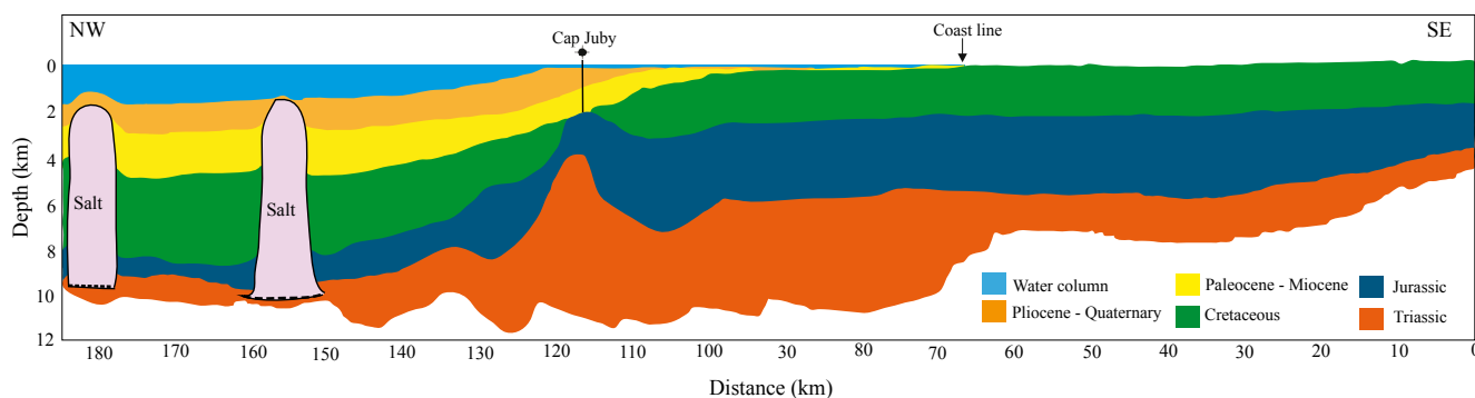
FIGURE 2. Cross section showing the extent of the onshore/offshore stratigraphy of the Tarfaya Basin (modified after Wenke, 2014), including Cap Juby well.
