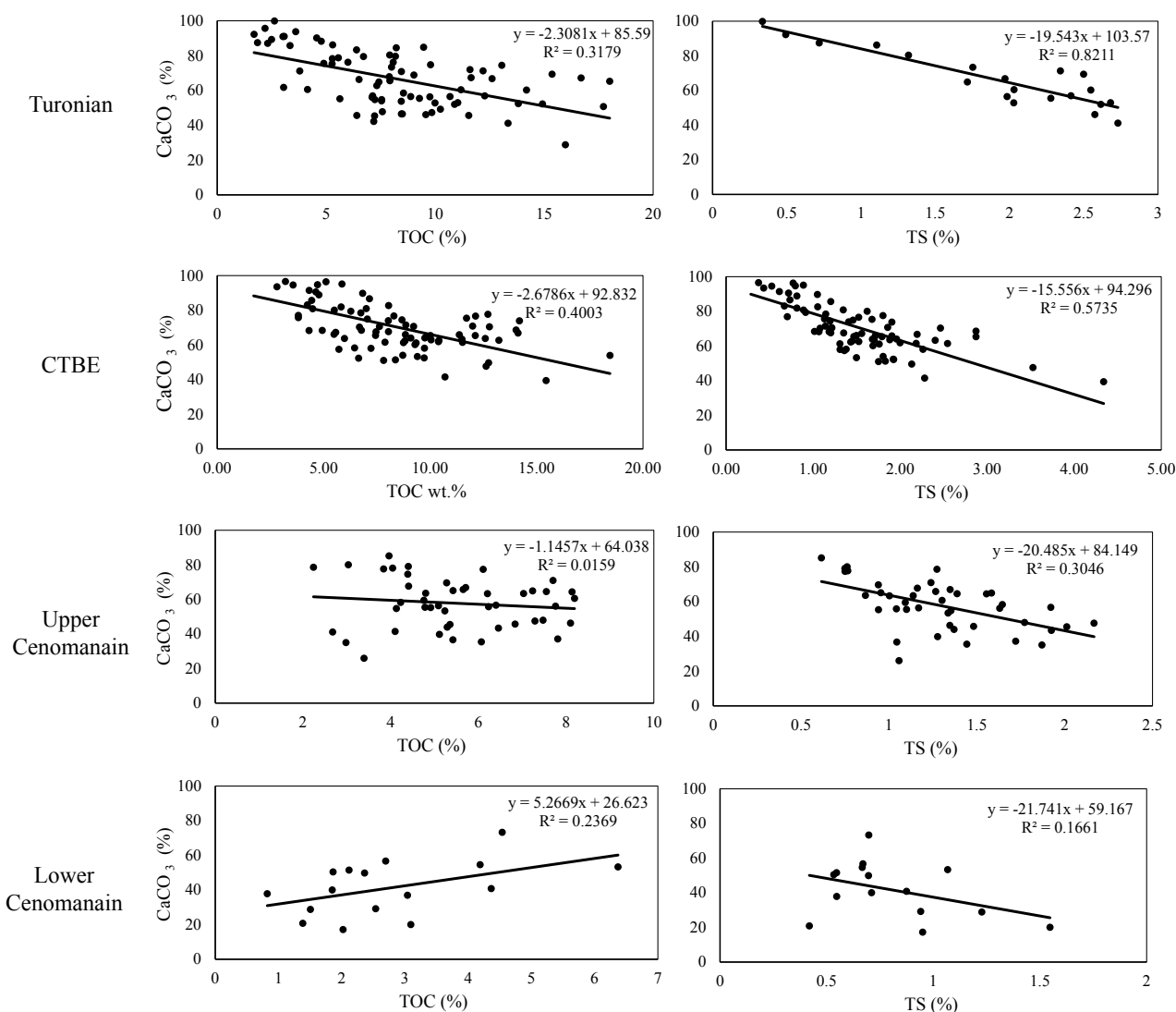
FIGURE 5. Cross plots between \text{CaCO}_3 versus TOC and TS. The correlation of \text{CaCO}_3 and TOC relationship changes significantly from positive in the Lower Cenomanian to negative in the Turonian. The \text{CaCO}_3 and TS correlations are always negative with variable regression coefficients.
