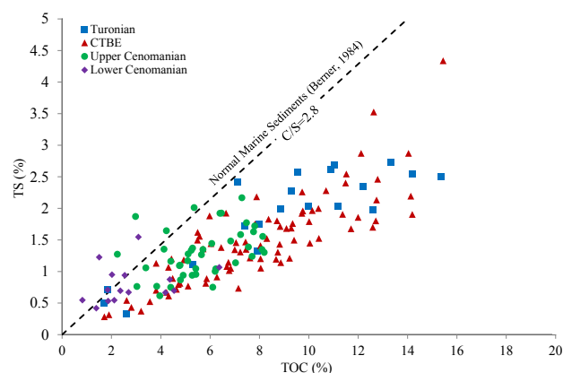
FIGURE 14. TS versus TOC cross-plot shows that the majority of the Cenomanian to Turonian samples are plotted below the normal marine line of Berner (1984) unlike the majority of the Lower Cenomanian samples which plot above the line.
