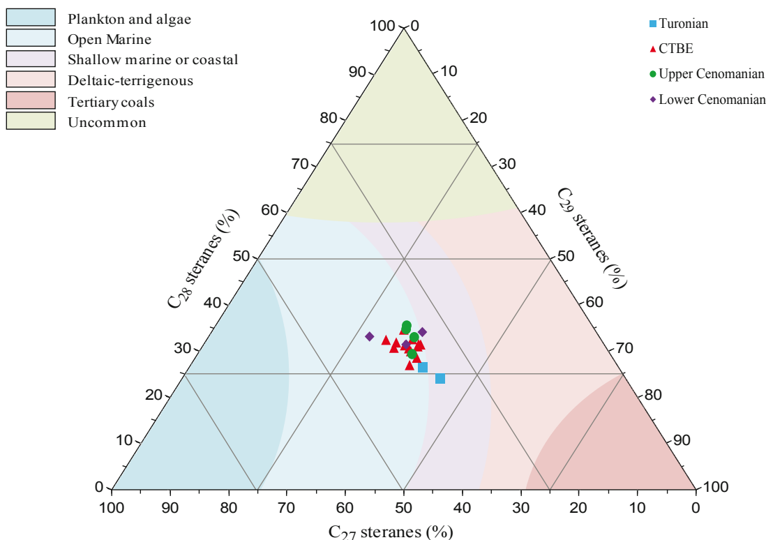
FIGURE 13. C_{27} - C_{29} steranes ternary diagram indicates shallow open marine depositional environment.
