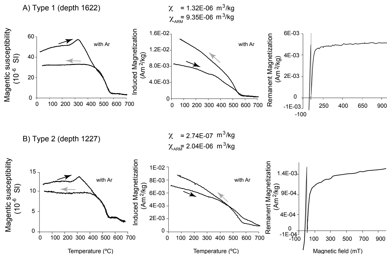
FIGURE 4. Rock magnetic analyses A) type 1 and B) type 2 of samples described in the text. From left to right: k-T curves (temperature dependent magnetic susceptibility), temperature dependent induced magnetization, and the isothermal remanent magnetization acquisition curve (right) with the back field (left).
