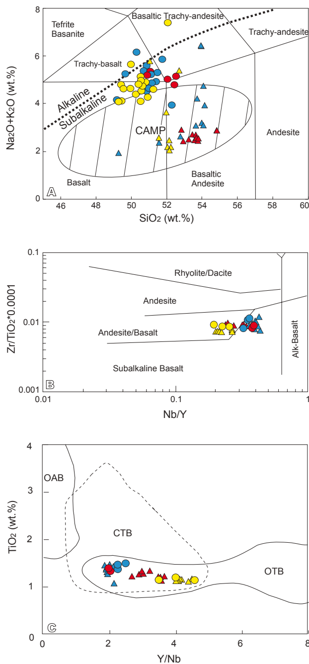
FIGURE 8. A) Total Alkali-Silica diagram (Le Bas et al. , 1986) for volcanic rocks from the Saharan Atlas. Data for CAMP domain after McHone (2000); B) Diagram of (Zr/TiO_2) \times 0.0001 versus Nb/Y (Winchester and Floyd, 1977) for volcanic rocks from the Saharan Atlas; C) Discrimination diagram TiO_2 versus Y/Nb (Floyd and Winchester, 1975) for volcanic rocks of the Saharan Atlas. OAB: Oceanic Alkali Basalts; CTB: Continental Tholeiitic Basalts; OTB: Oceanic Tholeiitic Basalts. Blue symbols: lower unit; red symbols: intermediate unit; yellow symbols: upper unit; circles: Saharan Atlas; triangles: Moroccan Atlas (from Marzoli et al. , 2004; Mahmoudi and Bertrand, 2007).
