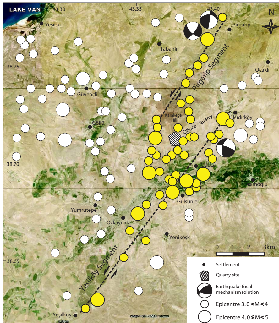
FIGURE 11. Earthquake records ( M \geq 3.0 ) in instrumental period near the Gülsünler fault (yellow circles showing earthquakes on the fault while white ones showing others) (KOERI, 2016).
