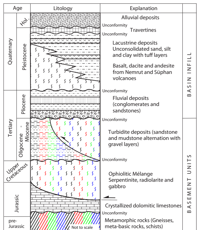
FIGURE 2. Tectono-stratigraphic chart of the study area (modified from Acarlar et al. , 1991; Şenel, 2008).
