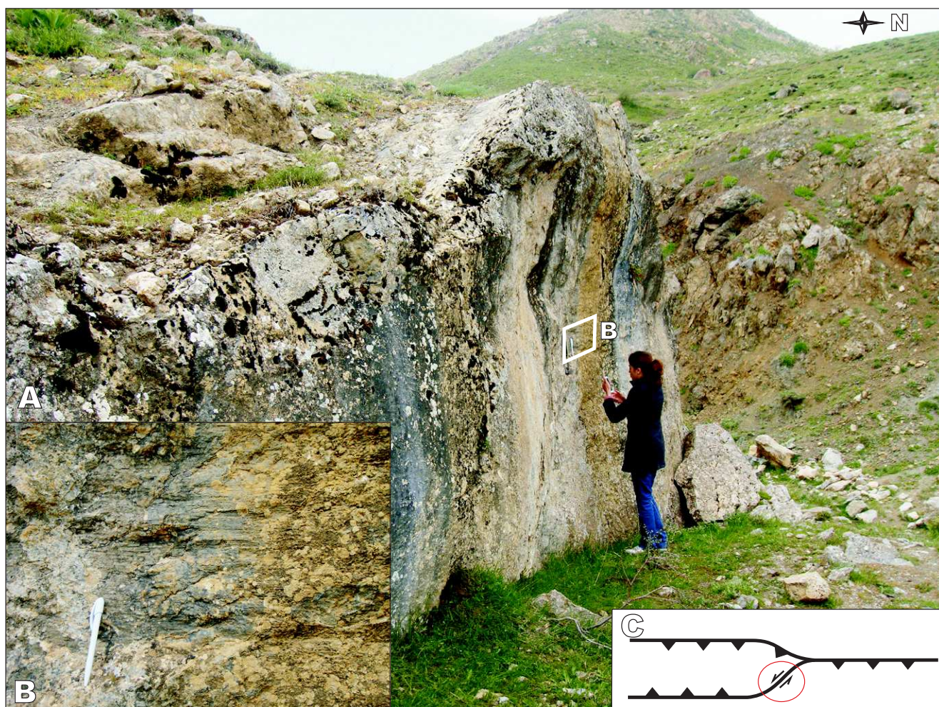
FIGURE 5. Field photograph of the eastern connection of the Özyurt thrust fault that has strike-slip character; A) vertical fault plane on Jurassic limestones, B) close-up view of fault plane and striations and C) plot of the fault plane (modified from Van der Pluijm and Marshak, 2004).
