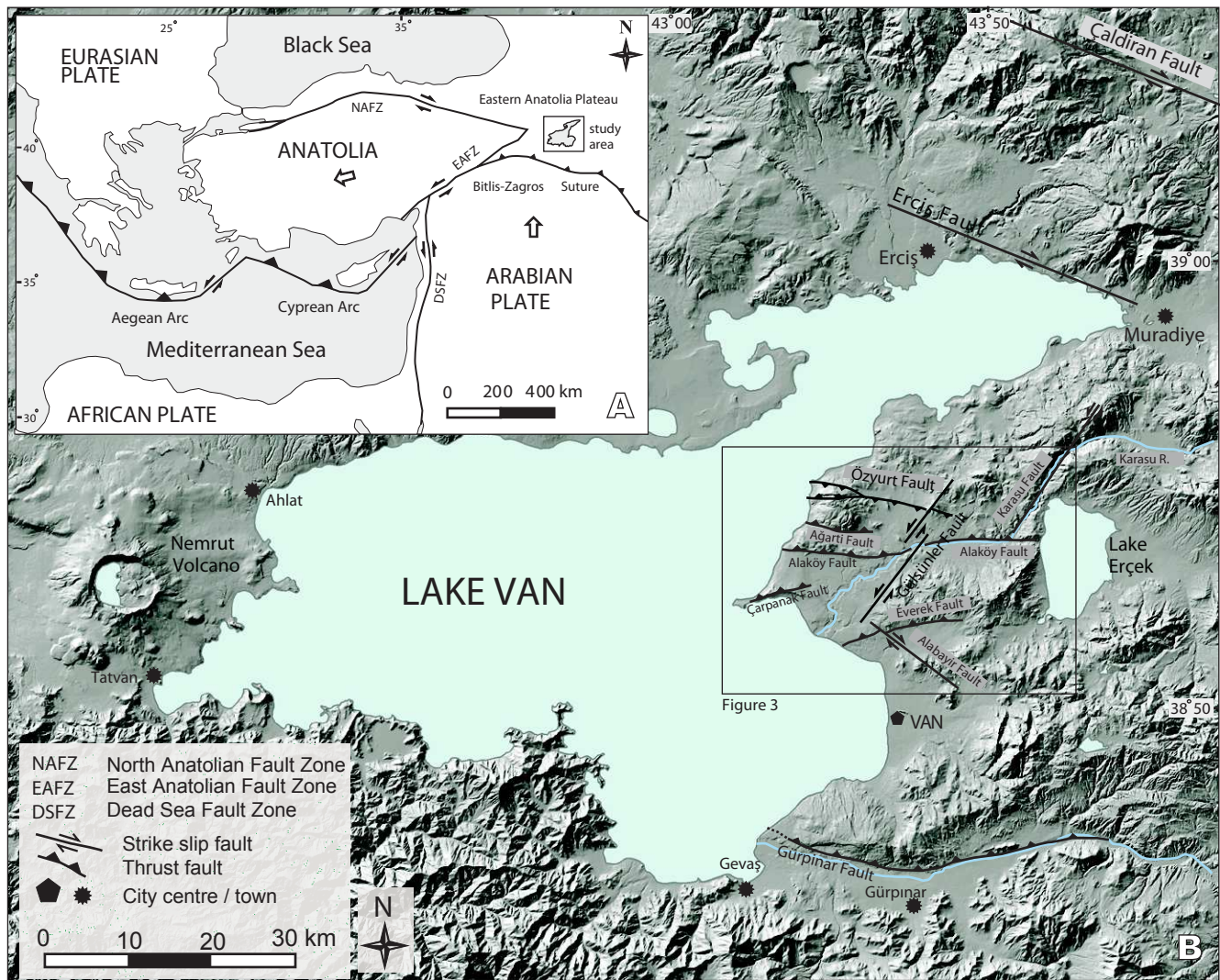
FIGURE 1. A) Major neotectonic features of Turkey and adjacent areas (white arrows indicate the motion of the plates), B) location map showing active faults on eastern part of Lake Van Basin.
