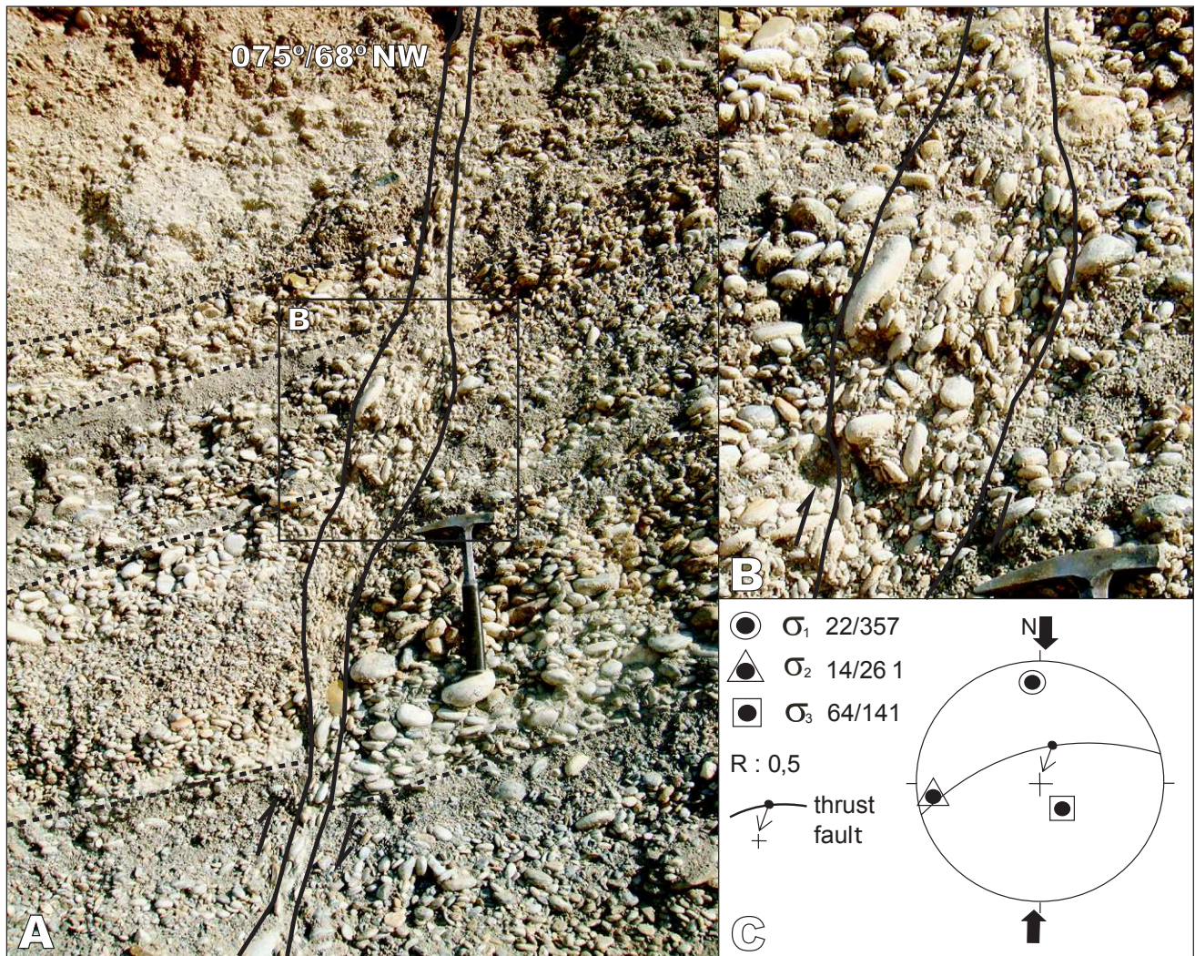
FIGURE 6. A) Field photograph showing the Özyurt fault in gravelly shore deposits of Lake Van, B) close-up view of fault zone (gravel orientations showing the direction of movement) and C) result of the palaeostress analysis on Schmidt lower hemisphere.
