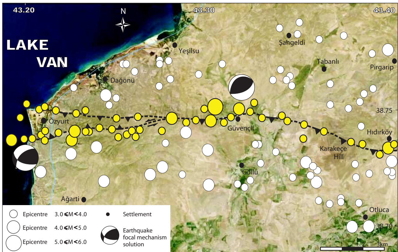
FIGURE 10. Earthquake records ( M \geq 3.0 ) in instrumental period near the Özyurt fault (yellow circles showing earthquakes on the fault while white ones showing others) (KOERI, 2016).
