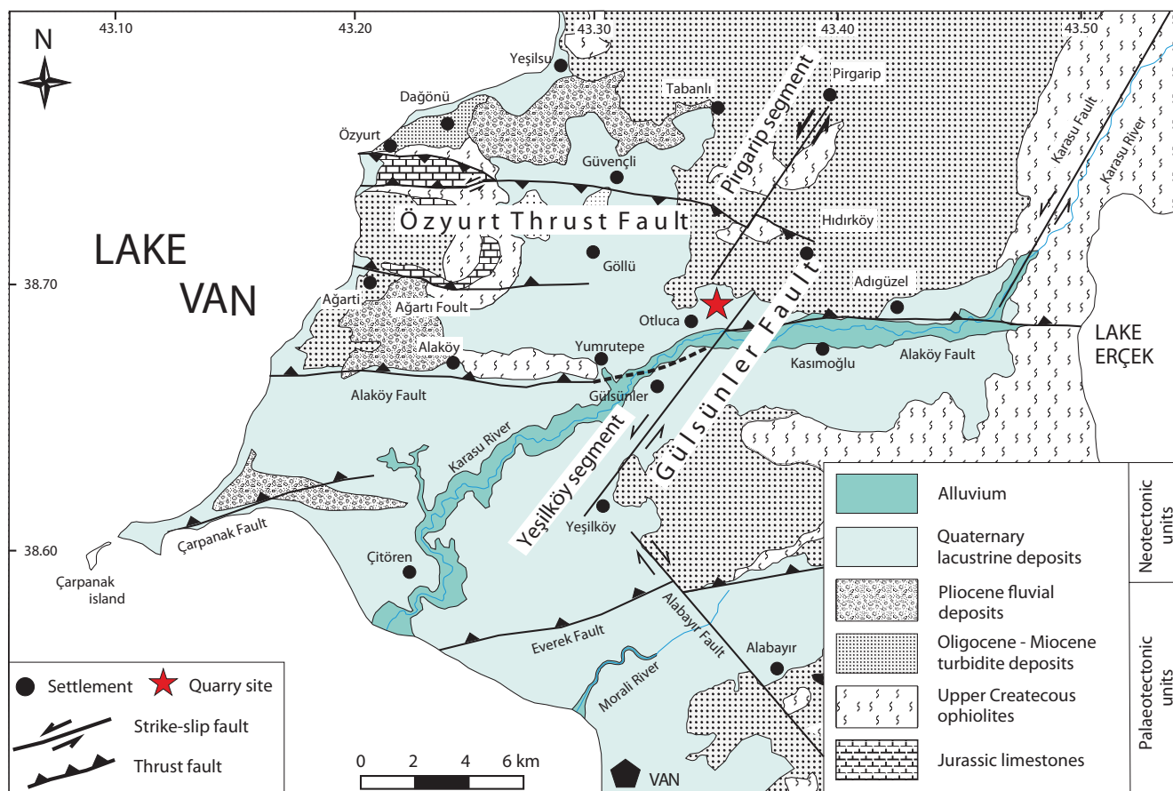
FIGURE 3. Geological map of the study area (modified from Acarlar et al. , 1991; Şenel, 2008).
