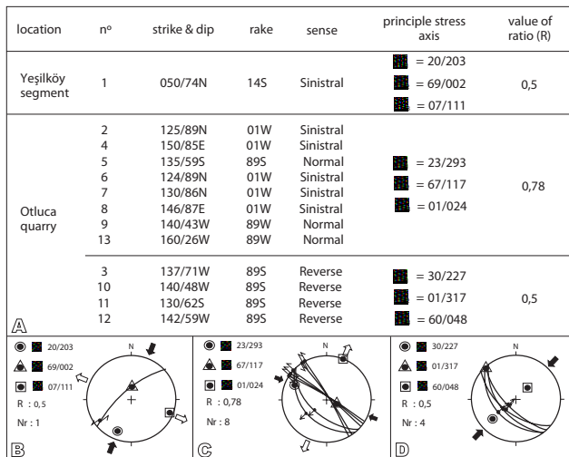
FIGURE 9. A) Fault-plane measurements on Yeşilköy segment and the north and west walls of the Otluca quarry. Results of the palaeostress analysis of striated fault planes with indications on Schmidt lower hemisphere; B) pure strike-slip stress regime, C) NE-SW tensional stress regime and D) NE-SW compressional stress regime.
