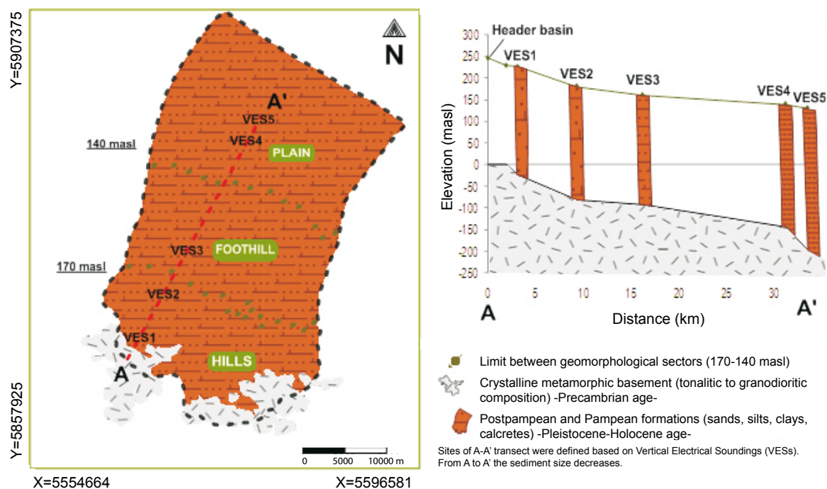
FIGURE 2. General geological characteristics and SW-NE cross section of the Languyú creek basin.
