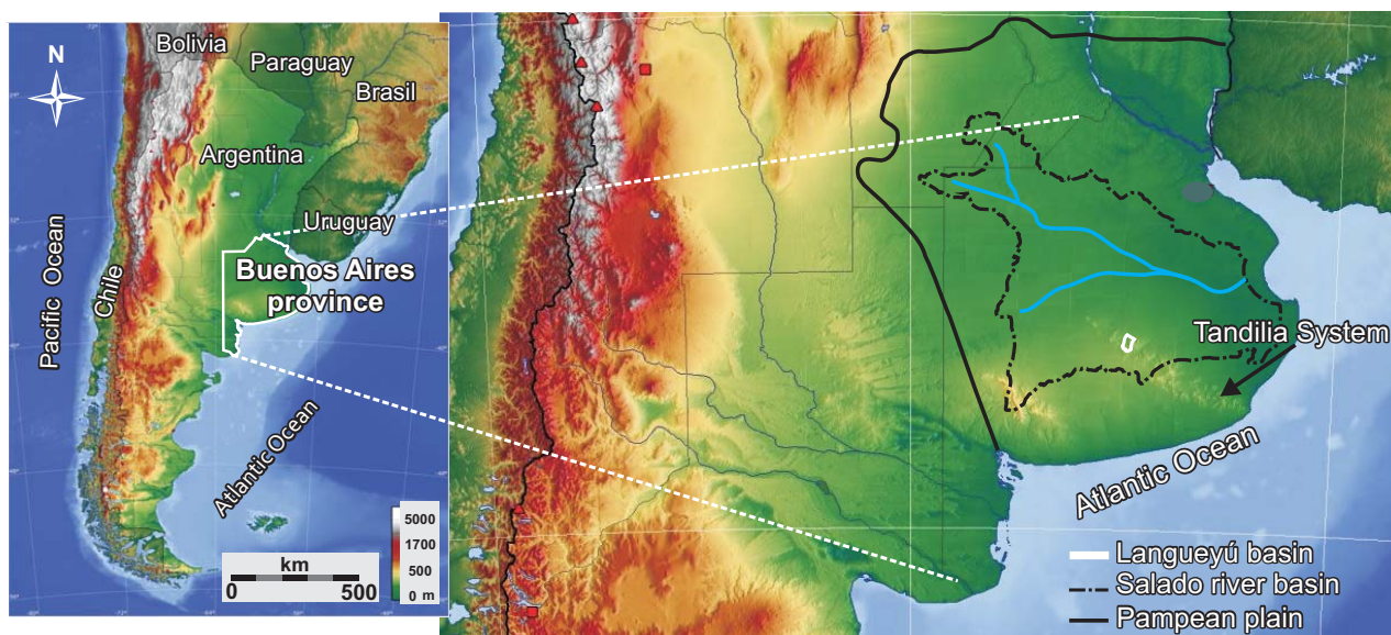
FIGURE 1. Location of the Languyú creek basin in Buenos Aires, Argentina.
