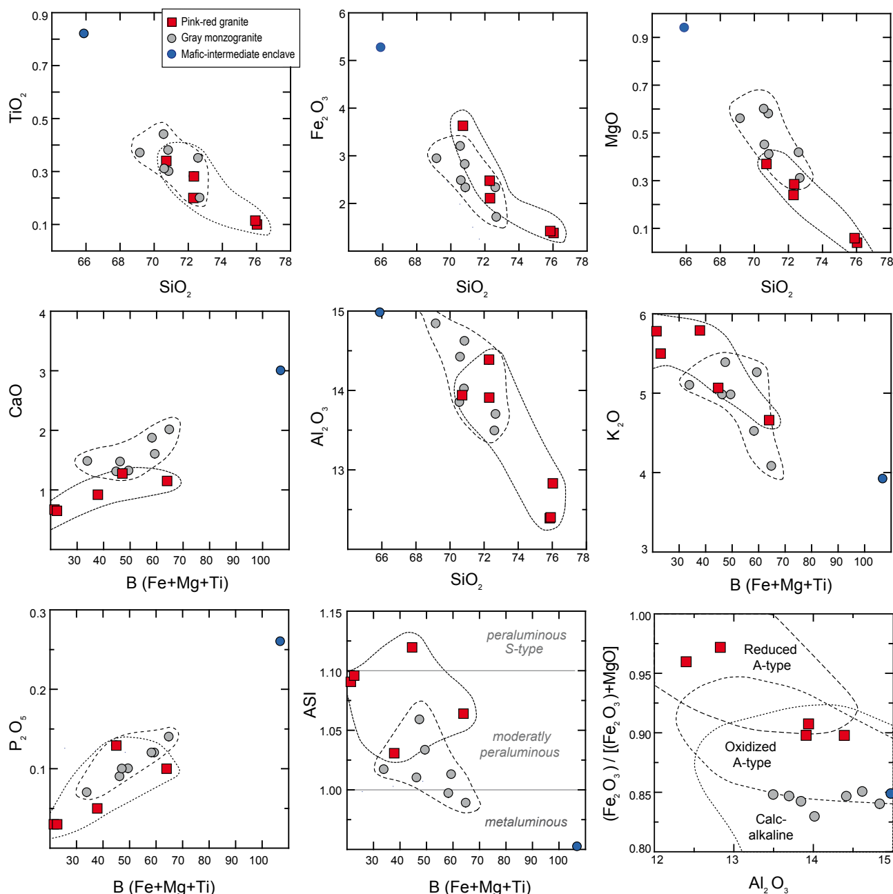
FIGURE 5. Geochemical variation diagrams for the major elements of the different granitoid units from the Porriño pluton. Both \text{SiO}_2 and the B parameter ( \text{Fe}+\text{Mg}+\text{Ti} , in molar proportions) are used as differentiation indexes. ASI is the alumina saturation index (or \text{A/CNK} ): \text{Al}_2\text{O}_3/(\text{CaO}+\text{Na}_2\text{O}+\text{K}_2\text{O}) in molar proportions. Fields in the last diagram after Dall'Agnol and Oliveira (2007).
