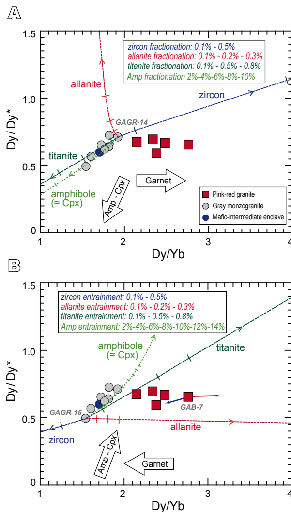
FIGURE 10. \text{Dy}/\text{Dy}^* vs. \text{Dy}/\text{Yb} diagram for representing REE pattern as a single point (Davidson et al. , 2014). Crystal fractionation (A) and crystal entrainment or accumulation processes (B) were modeled using standard mass balance equations (Ragland, 1989). The mineral phases used in the modeling are: amphibole from Table I; zircon and titanite from Pe1 granodioritic orthogneiss (Gregory et al. , 2009); and allanite from Pe11 granodioritic migmatite (Gregory et al. , 2009). Arrows of amphibole/clinopyroxene and garnet are from Davidson et al. (2014). GAGR-14: starting composition for the fractionation models. GAGR-15 and GAB-7: starting compositions for the entrainment models.
