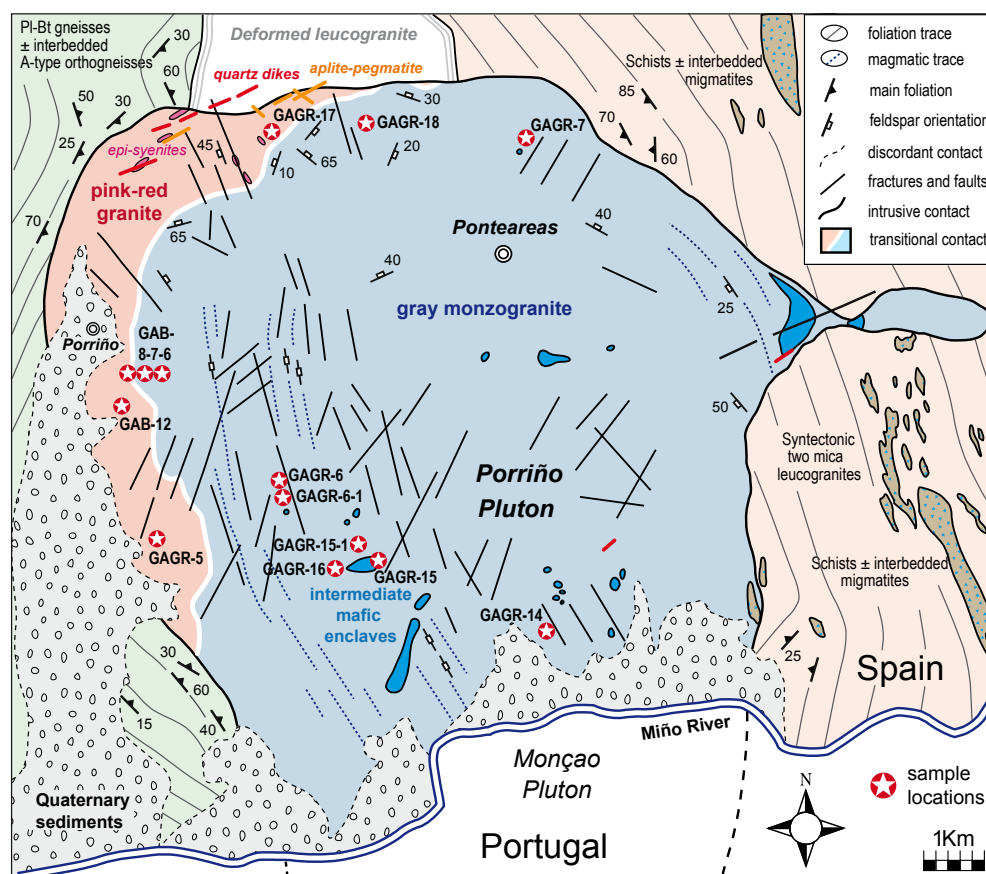
FIGURE 2. Modified geological map (after Corretgé et al. , 1981 and Barrera Morate et al. , 1989) of the post-tectonic Variscan Porriño pluton, including field observations and sample locations.
