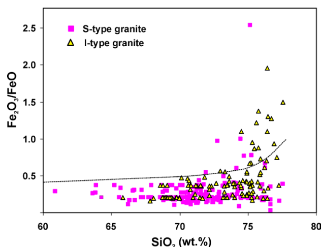
FIGURE 3. SiO 2 versus ferric/ferrous ratio of SCS granites. Whole-rock granite chemical data with ferrous iron determined by titration with a standardised potassium permanganate solution are from Bellido (1979), Casillas (1989), Andonaegui (1990) and Pérez-Soba (1991). Broken line is the separation line between magnetite- and ilmenite-series (Ishihara et al. , 2000).
