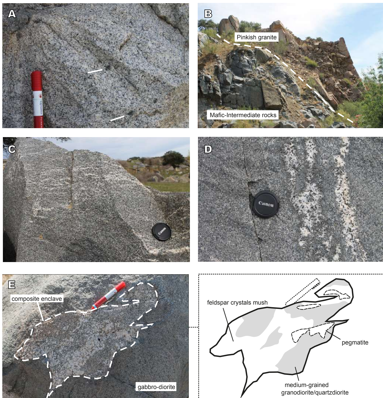
FIGURE 3. Representative field relationships of the main rock types of the Santa Eulália-Monforte massif: A) greyish granite from the core, containing megacrysts of cordierite; B) sharp contact between the coarse-grained pinkish granite and the mafic-intermediate rocks from the external ring, C) intermediate (dioritic) and D) mafic (gabbroic) bodies from the external ring, with leucocratic veins; E) composite enclave with irregular shape consisting of medium-grained quartzdiorite/granodiorite, coarse-grained K-feldspar mush and pegmatite, surrounded by gabbro-dioritic rocks.
