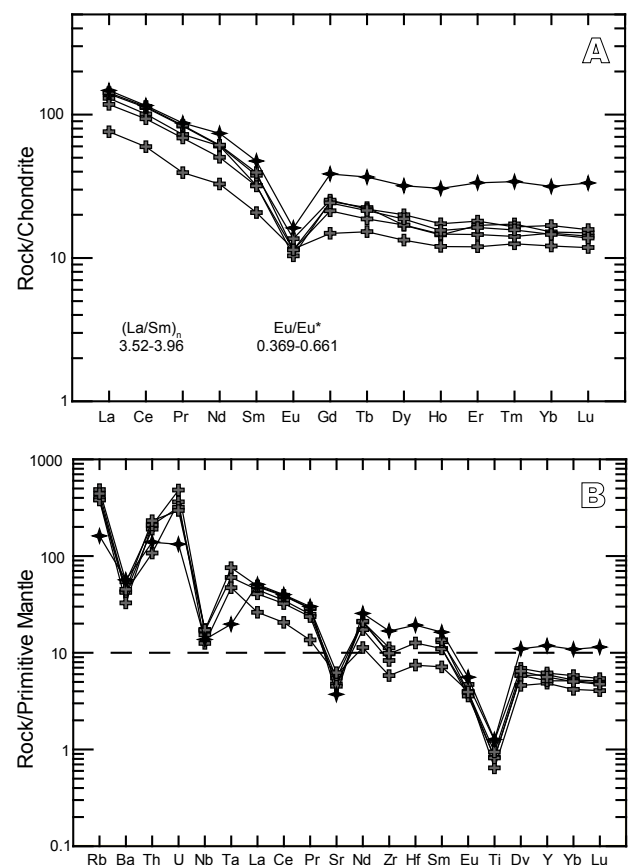
FIGURE 7. Multi-element diagrams showing the comparison between the El Crispinejo granite and the trondhjemitic granites of the SPZ. A) Chondrite-normalized Rare Earth element pattern. B) Primitive mantle-normalized trace element pattern. The crosses represent samples from the El Crispinejo granite. The four-point start pattern represents an average value of the trondhjemitic granite of the SPZ. Normalizing values after Sun and McDonough (1989).
