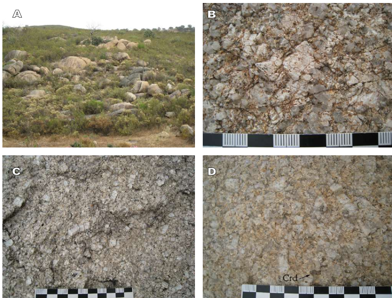
FIGURE 3. Outcrop and macroscopic aspect of the El Crispinejo granite. A) General outcrop, boulder field characteristic of the coarse-grained granite. B) Macroscopic texture of granite with large quartz and feldspar crystals (scale major unit: cm, minor unit: mm). C) Porphyritic facies with K-feldspar megacrysts. D) Macroscopic texture of granite with cordierite prisms (Crd).
