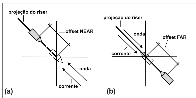
Figura 2 - Casos de análise colineares, offsets NEAR e FAR. (a) caso NEAR colinear; (b) caso FAR colinear.
