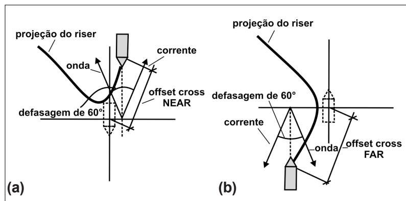
Figura 4 - Casos de análises, offsets cross NEAR e cross FAR. (a) caso CROSSED NEAR CROSS; (b) caso CROSSED FAR CROSS.
