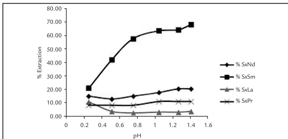
Figure 2 Extraction efficiencies of La(III), Pr(III), Nd(III) and Sm(III) from system DEHPA-Isoparaffin 17/21 at different initial pH.
