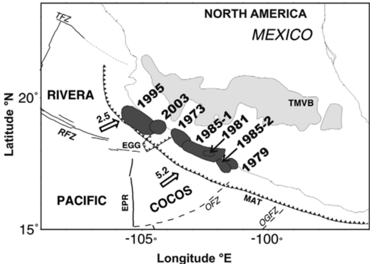
Fig. 1. Tectonic map of the Cocos (COCOS) and Rivera (RIVERA) plates in the Mexican subduction zone and the rupture fault zones of the 7 large earthquakes studied, inferred from their aftershock areas. NORTH AMERICA=North American Plate; PACIFIC=Pacific Plate; RFZ=Rivera Fracture Zone; EPR=East Pacific Rise; EGG=El Gordo Graben; MAT= Middle American Trench. Numerals indicate the year of occurrence of these earthquakes.
