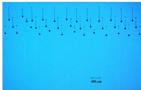
FIGURE 8. Figure caption.(Colour online) Shadowgraph picture of droplets jetted from a Xaar XJ126 printhead. The droplets travel at an speed of 5 m/s and have a volume of 80 picoliters.
