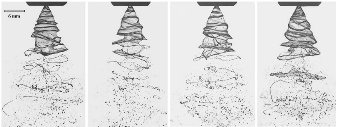
FIGURE 5. (Colour online) Shadowgraph images of quenching oil at 38°C emerging from a 1.2 mm atomizer nozzle. The average terminal speed of the spray droplets is 15 m/s.
