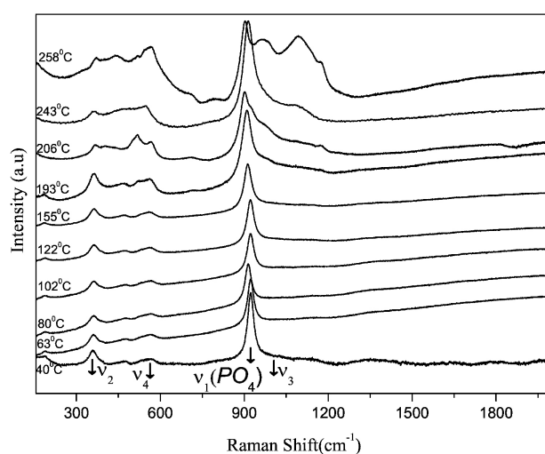
FIGURE 6. Raman spectra of the \text{KADP}_{0.1} crystal at different temperatures. The arrows indicate the evolution of the selected modes with temperature. The modes are assigned in correspondence with Ref. [14] and [17].
