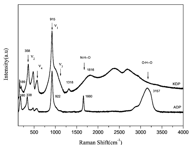
FIGURE 2. Raman spectra at room temperature of KDP and ADP crystalline compounds. The arrows indicate the location of the modes in correspondence with Ref. [14] and [17].
