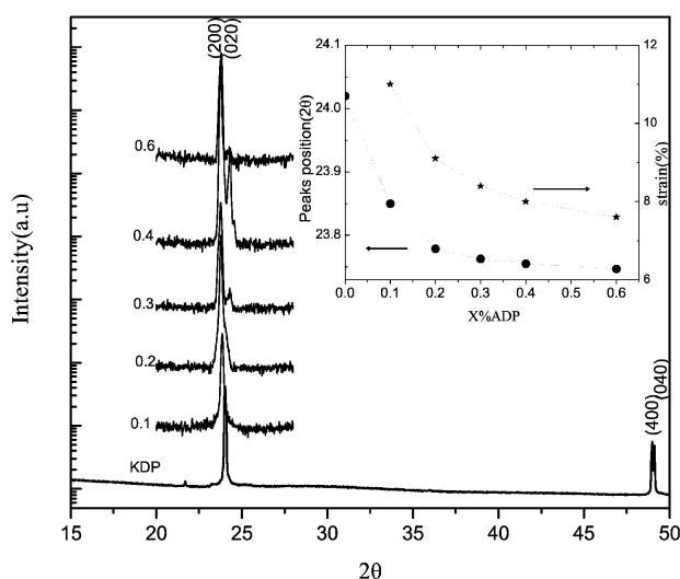
FIGURE 1. X-ray diffraction at room temperature of KADPx-system for: x = 0.0, 0.1, 0.2, 0.3, 0.4 and 0.6 . For x > 0 , only the most intense peak (200) are shown for data analysis (see text). The inset shows the dependence of the peak position and strain with concentration. The dashed line is a guide to the eye.
