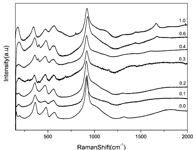
FIGURE 7. Raman spectra of KADPx crystals with x=0.0, 0.1, 0.2, 0.3, 0.4, 0.6 , and 1.0 , at temperature of 151^\circ\text{C} . The compounds retain the vibrational bands that are present in the low temperature region.
