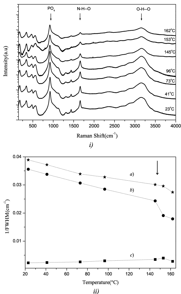
FIGURE 5. i) Raman spectra of ADP-crystal at different temperatures. The arrows indicate the modes associated with stretch vibrations of \text{PO}_4 and N-H-O and O-H-O species, respectively. ii) Temperature dependence of FWHM for the peaks located at: a) 922 \text{cm}^{-1} , b) 1660 \text{cm}^{-1} and c) 3157 \text{cm}^{-1} of the ADP crystal. The arrow indicates the transition region that shows an abrupt change of FWHM. The dashed lines are a guide to the eye.
