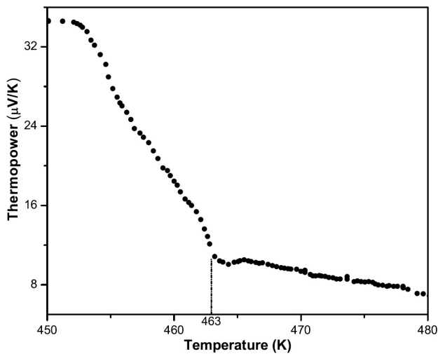
FIGURE 1. Temperature dependence of the thermoelectrical power of almel close to the ferromagnetic-paramagnetic phase transition.
