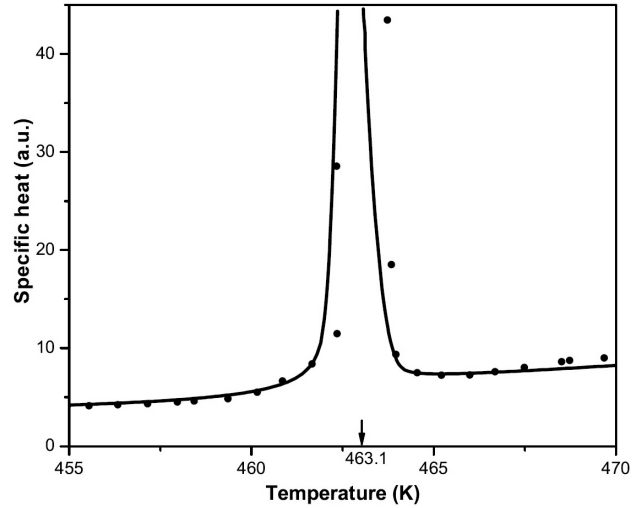
FIGURE 2. Temperature dependence of specific heat c_P(T) under normal pressure as a function of temperature for an sample of almel, which shows a sharp peak at T_C = 463 K.
