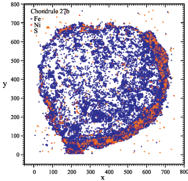
Figure 3. Metal boundaries inside c27b chondrule, determined using an image processing technique, focusing in the nickel, iron and sulphur elements. C27b is an example of an iron-rich chondrule with iron- and nickel-rich rim.
