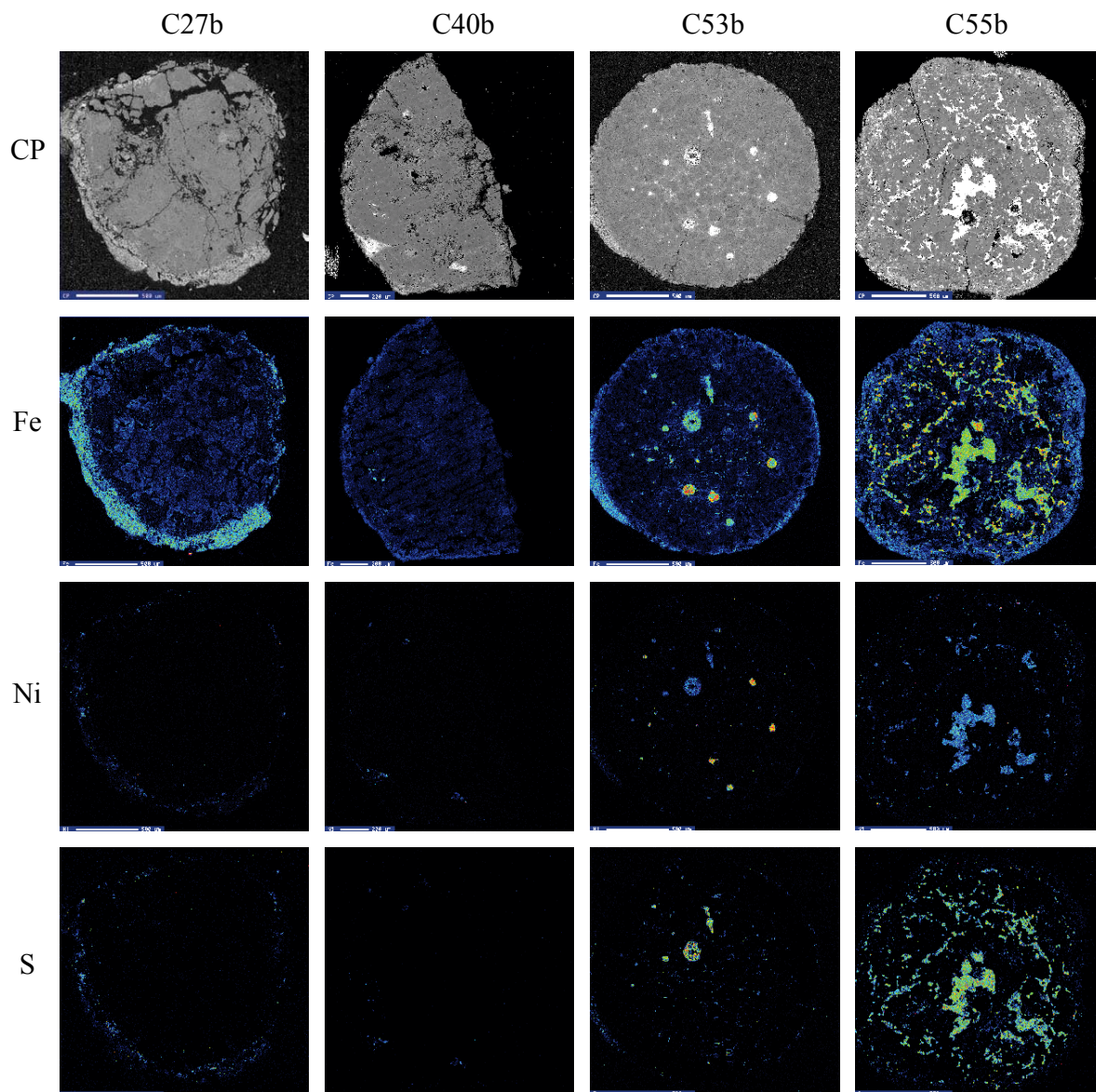
Figure 2. Scanning electron microscopy (SEM) and SEM-Energy dispersive spectroscopy (EDS) images for individual chondrules from Allende meteorite. SEM composite pictures (CP) and false color compositional images for Fe, Ni and S are shown for chondrules c27b, c40b, c53b and c55b (see text for description).
