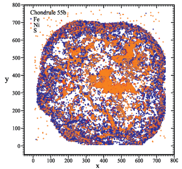
Figure 6. Metal boundaries inside c55b chondrule, determined using an image processing technique, focusing in the nickel, iron and sulphur elements. C55b is an example of iron-, nickel- and sulphur-rich chondrules. Note the internal mineralogical assemblage and spatial arrangement, with sulphur-rich minerals.
