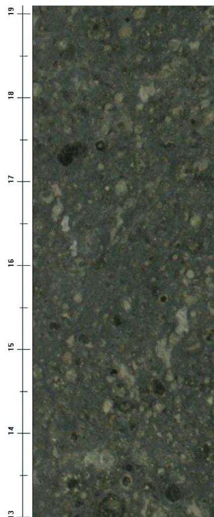
Figure 1. Fragment of the Allende carbonaceous chondritic meteorite (6 cm slab cut from Allende showing distribution of chondrules and refractory inclusions in the fine grained silicate matrix).
