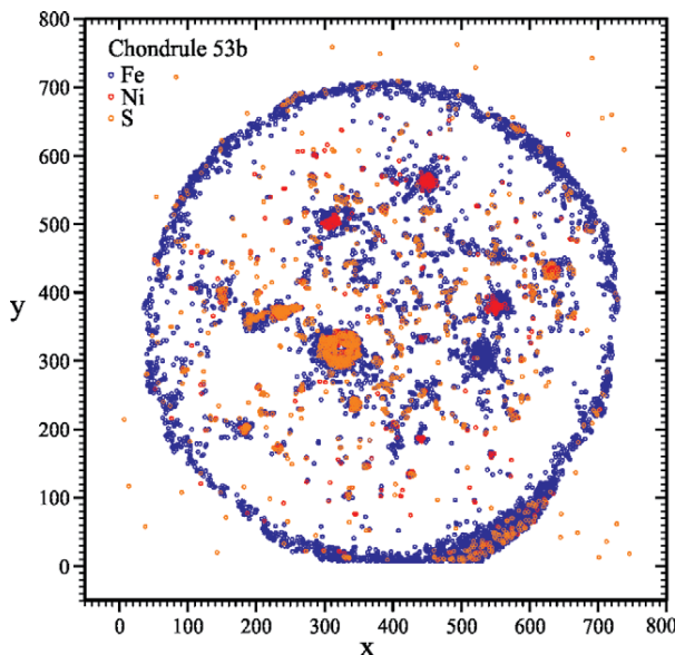
Figure 5. Metal boundaries inside c53b chondrule, determined using an image processing technique, focusing in the nickel, iron and sulphur elements. C53b is an example of iron- and nickel-poor chondrules with iron-rich rims. Observe the nickel and sulphur rich metallic inclusions.
