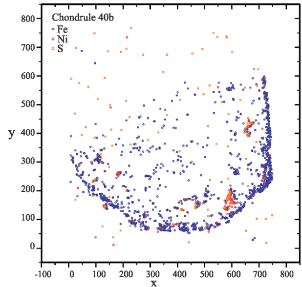
Figure 4. Metal boundaries inside c40b chondrule, determined using an image processing technique, focusing in the nickel, iron and sulphur elements. C40b is an example of iron-, nickel- and sulphur-poor chondrules.
