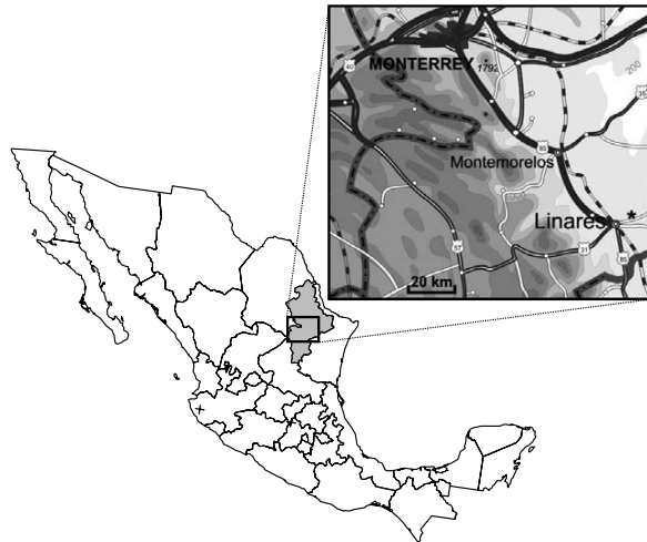
Figure 1. Map of Mexico and detail of south Nuevo León; the area of the find is shown by an asterisk.
