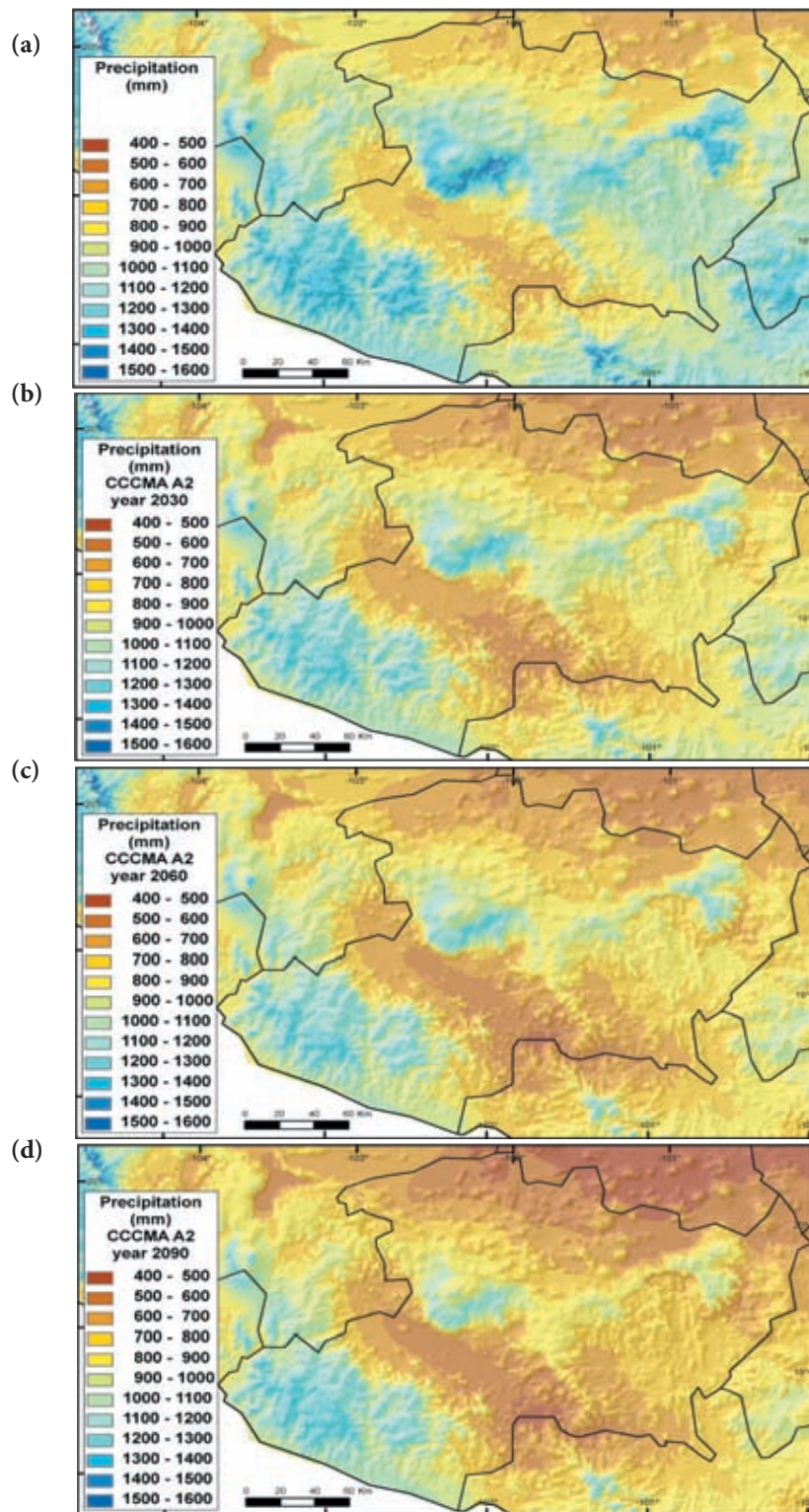
Figure 7. Mapped predictions for mean annual precipitation (mm), for contemporary (a), decades centered in the year 2030 (b), 2060 (c) and 2090 (d) climates, using output from the Canadian Center for Climate Modeling and Analysis model, scenario A2.
