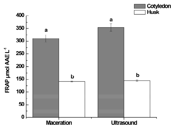
Fig. 4. Antioxidant capacity of cocoa extracts measured by FRAP assay. Concentration of sample was 0.10 mg mL -1 . Values are expressed as mean \pm sd ( n = 3 ). Means with different letters were significantly different ( P < 0.05 ).
