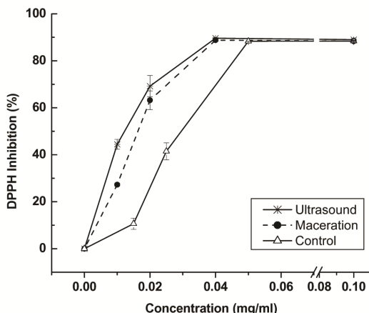
Fig. 3. Scavenging effect of cocoa cotyledon extracts on DPPH radicals. Values are expressed as mean \pm sd ( n = 3 ). Ascorbic acid was used as the control.
