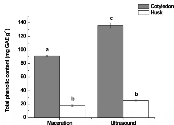
Fig. 1. Total phenolic content of cocoa extracts. Values are expressed as mean \pm sd ( n = 3 ). Means with different letters were significantly different ( P < 0.05 ).
