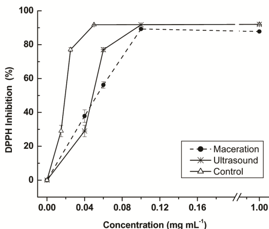
Fig. 2. Scavenging effect of cocoa husk extracts on DPPH radicals. Values are expressed as mean \pm sd ( n = 3 ). Ascorbic acid was used as the control.
