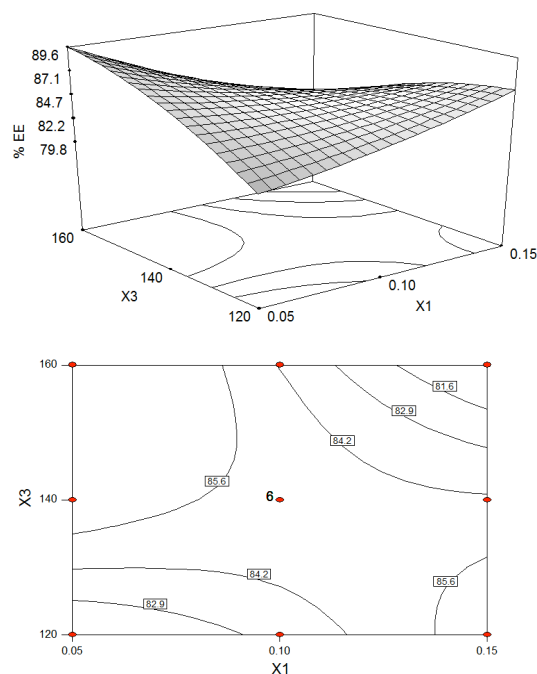
Fig. 3. The (a) 3D response and (b) 2D contour plots of the EE % affected by volumetric dispersed phase ( X_1 ) and drying air inlet temperature ( X_3 ).
