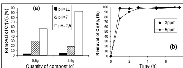
Figure 5. a) Effect of pH on Cr(VI) elimination using two quantities of compost 1 ( \text{Cr(VI)} = 5 \text{ mg L}^{-1} initial concentration). b) Determining equilibrium time for Cr(VI) adsorption on compost. 1. 3 \text{ mg L}^{-1} and 5 \text{ mg L}^{-1} initial Cr(VI) concentrations, 2.5 g compost and pH=2.5. 100 mL volume and 150 rpm stirring were used in both experiments.
