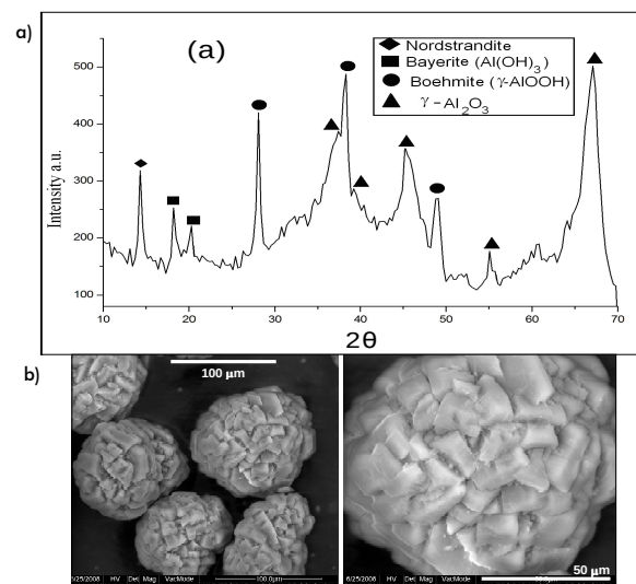
Figure 1. X-ray diffraction pattern (a) and SEM images (b) of the alumina used as adsorbent
