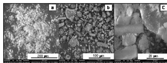
Figure 2. SEM microographies of compost 1 before removal of chromium (VI). a) 600X, b) 1,000X, c) 4,000X.
