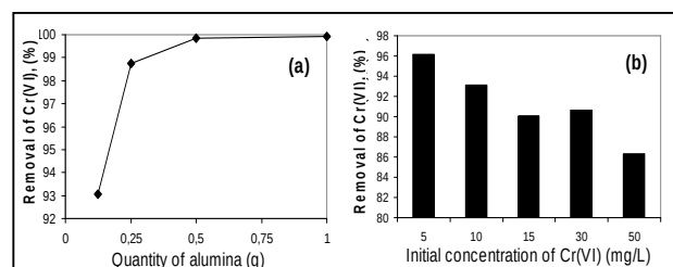
Figure 4. a) Effect of adsorbent amount on chromium (VI) adsorption on alumina using \text{Cr(VI)} = 10 \text{ mg L}^{-1} initial concentration. b) The effect of initial Cr(VI) concentration using 0.25g alumina. A 1 hour contact time, 25mL solution volume, pH=2 and 150 rpm stirring conditions were used in both experiments.
