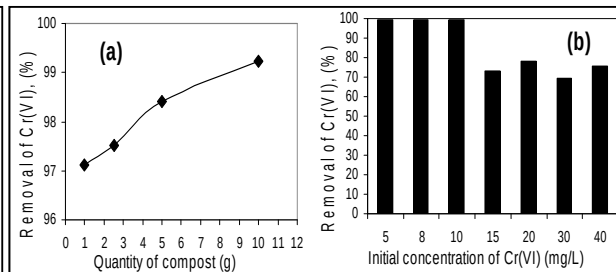
Figure 6. a) The effect of compost 1 quantity on Cr(VI) removal (Cr(VI) = 5 \text{ mg L}^{-1} initial concentration). The effect of initial Cr(VI) concentration on its removal from aqueous solution using compost 1 (2.5 g compost). In both experiments: 100 mL solution, pH=2.5, 150 rpm stirring for 3h).
