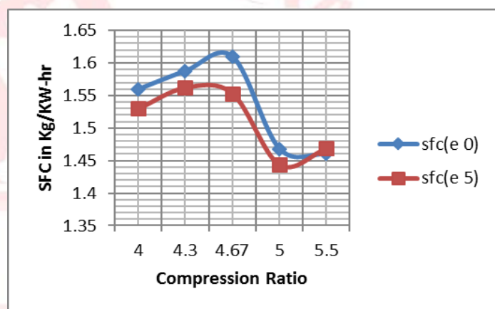
Fig 5. Comparison of SFC with CR for E0 & E5 blends
