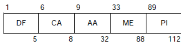
Figura 9. Trama ADS-B.
